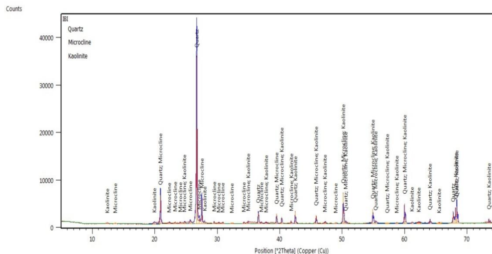
Figure 2: XRD MEASUREMENT FOR IBI SOILS
