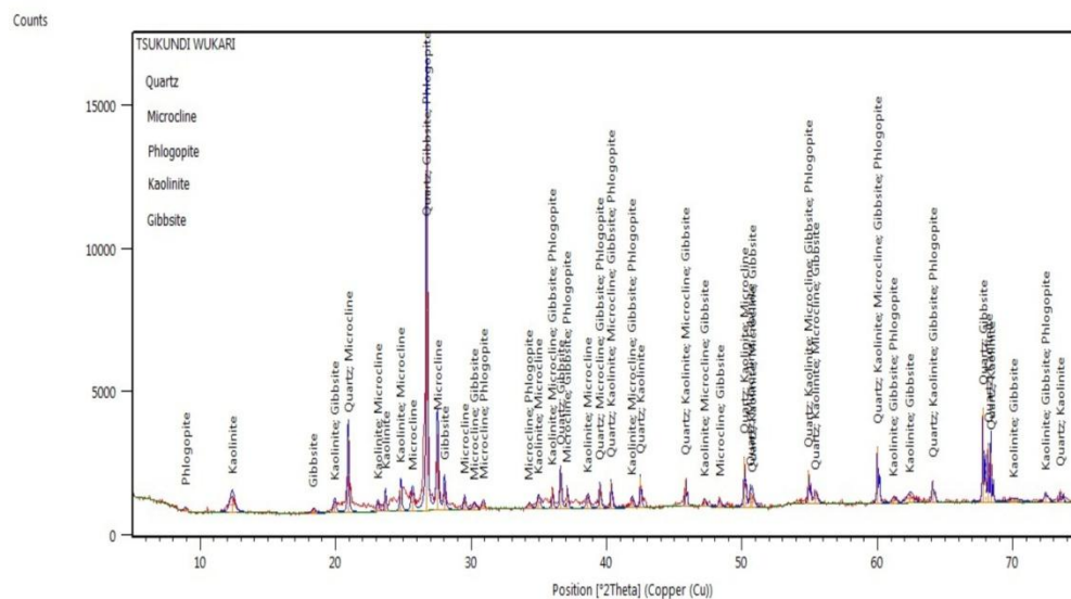
Figure 3: XRD MEASUREMENT FOR WUKARI SOIL
