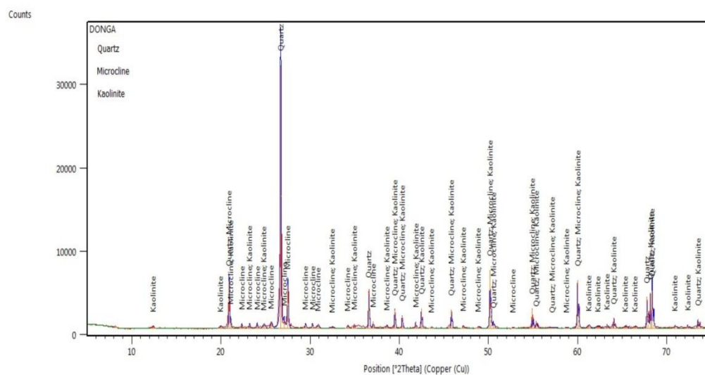
Figure 4: XRD MEASUREMENT FOR DONGA SOILS
