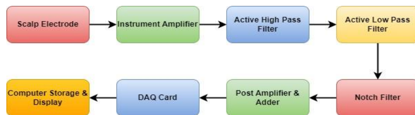
Figure 2: EEG Acquisition Process
