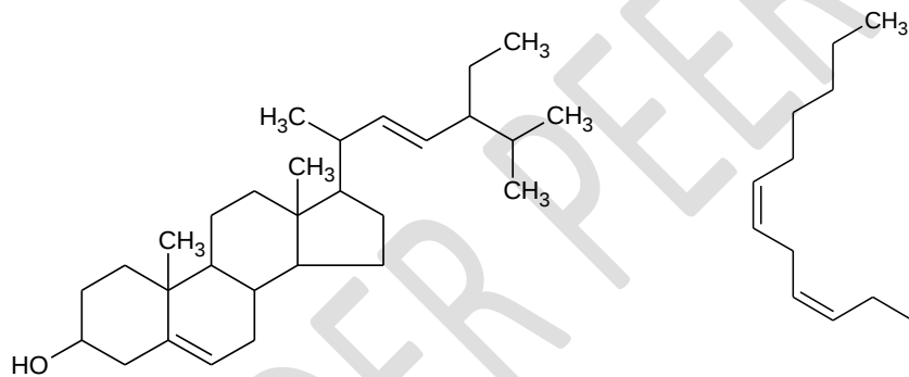
Stigmasterol
