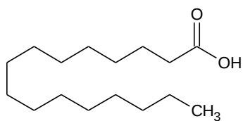
n-hexadecanoic acid
