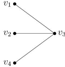
Figure 2: Claw graph
