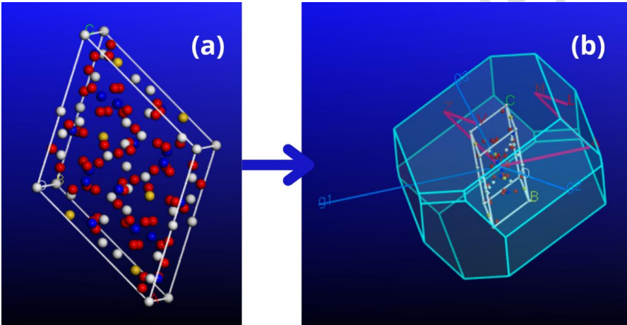
Fig. 1.(a) Crystal structure of gold nitrate (AuH7N4O15), (b) primitive structure of gold nitrate with the representation of the Brillouin zone, including its high-symmetry points and primitive vectors.
