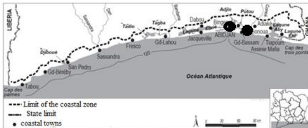
Fig. 1. Map showing the delimitation of the Côte d'Ivoire's coastline with landing sites (●) source: Pottier and Anah (2008)
