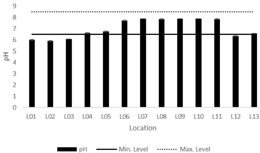
Figure 5 - Variation in pH of the water samples collected from the locations L01 to L13
