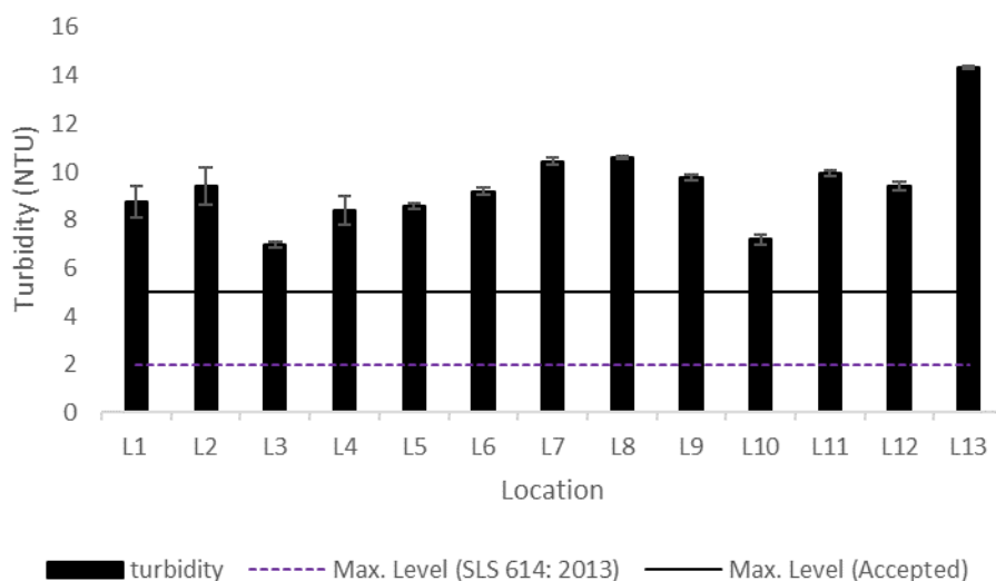
Figure 2. Turbidity of water samples collected from the locations L01 to L13
