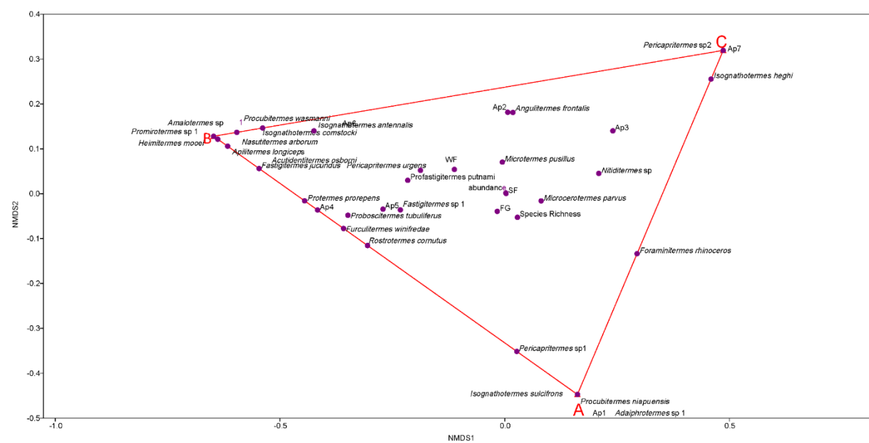
Figure 5: NMDS analysis of the different slope gradients based on the Composition of termites assemblages (FG: fungus growers, SF: soil Feeding; WF: wood feeding)
