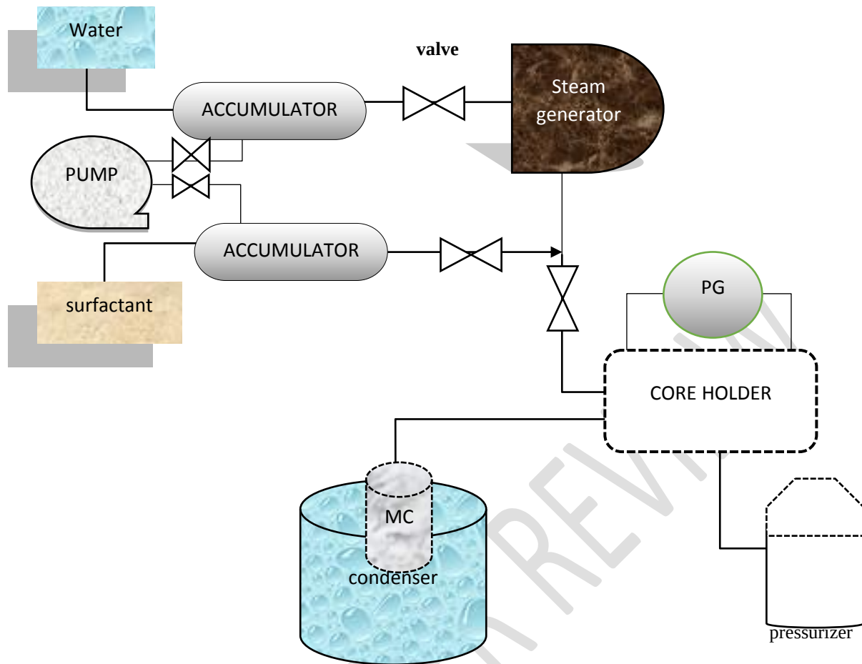
Figure 6: Core Flooding Schematic diagram of experimental setup
