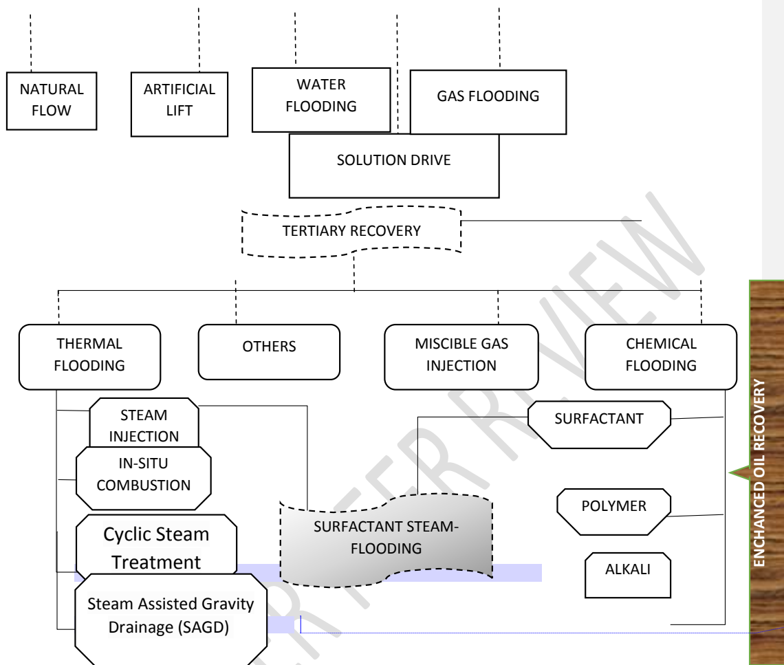
Figure 1: Enhanced Oil Recovery of surfactant-steam-flooding
