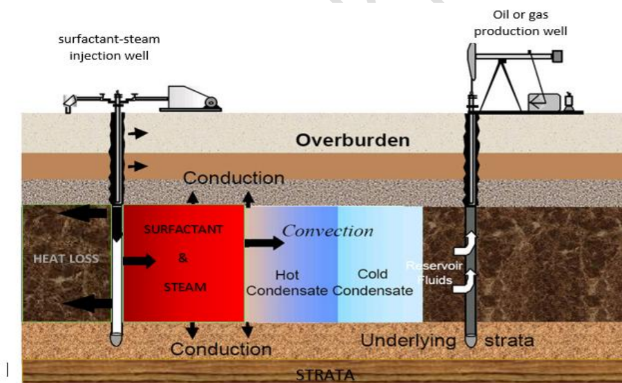
Figure 4: STEAM-DRIVE OIL RECOVERY MECHANISM
