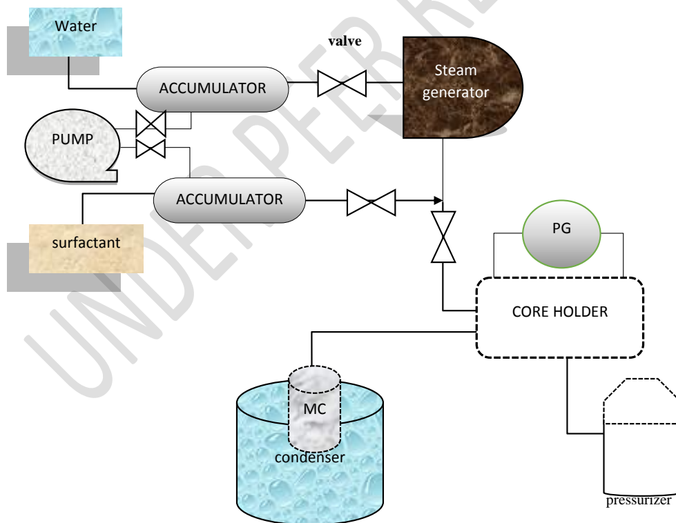
Figure 6: Core Flooding Schematic diagram of experimental setup
