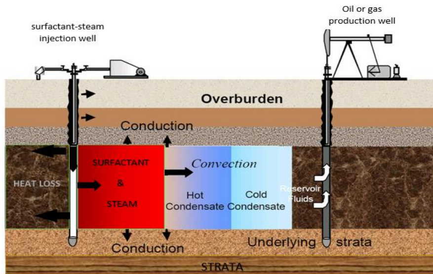
Figure 4: STEAM-DRIVE OIL RECOVERY MECHANISM
