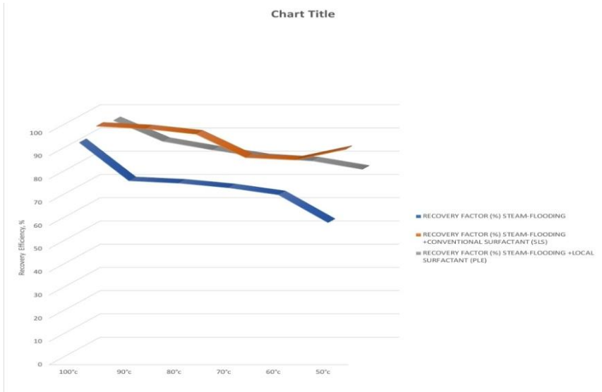
Figure 8: chart showing a comparison of the effect of temperature of the recovery efficiency of steam-flooding with the Steam-flooding Surfactant
