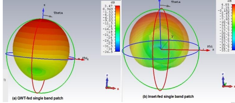
Figure.26. 3-D gain of single band antenna at 2.4 GHz
