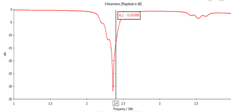
Fig. 15. Return Loss plot of 1 × 4 series-fed antenna array at 2.4 GHz
