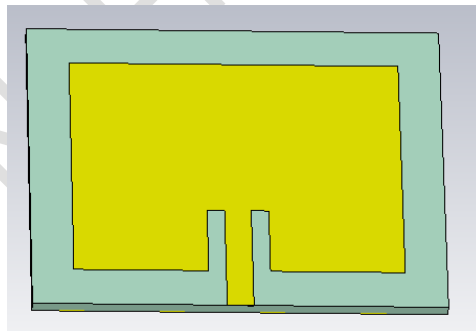
Fig. 6. Model of 2.4 GHz inset-feed Single Band MSA in CST studio
