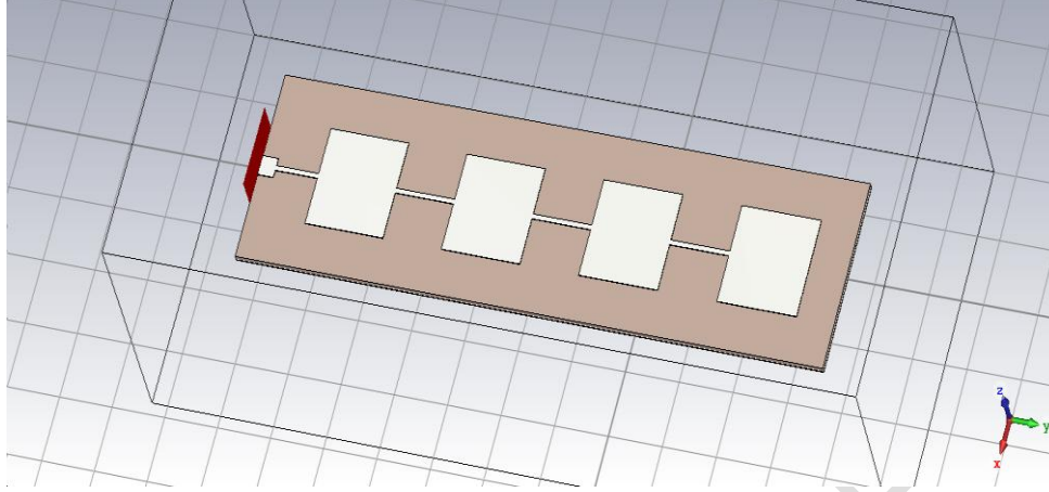
Fig. 4. Model of series-fed 1 x 4 patch MSA array
