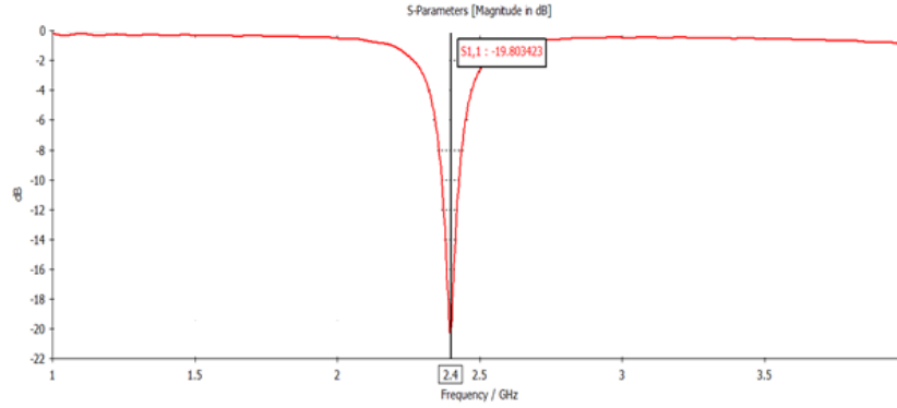
Fig. 14. Return Loss plot of the quarter-wave-fed single-band antenna at 2.4 GHz
