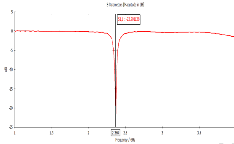
Fig. 17. Return loss plot of the proposed 1 × 2 cooperate-fed antenna array
