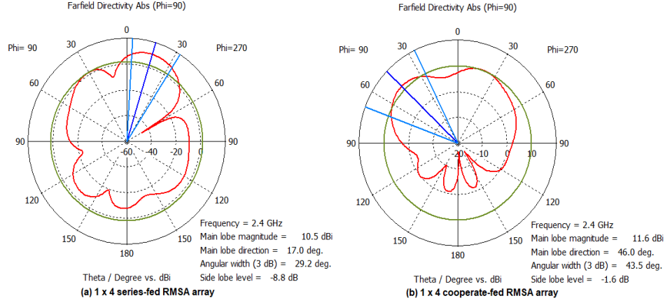
Fig.21. Directivity of proposed antenna arrays at 2.4 GHz in H-plane ( \phi = 90^\circ )
