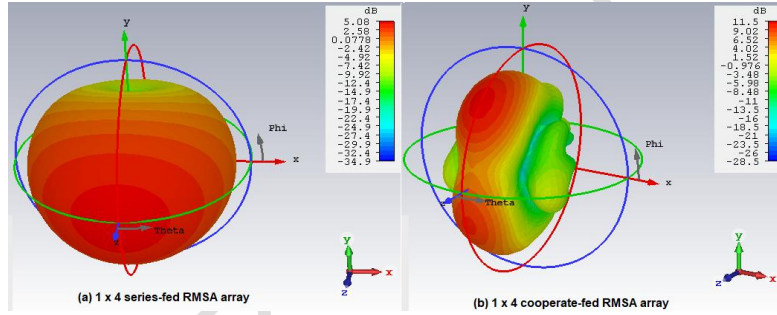
Fig.27. 3-D gain of proposed 1 \times 4 series-fed and 1 \times 4 cooperate-fed RMSA array at 2.4 GHz
