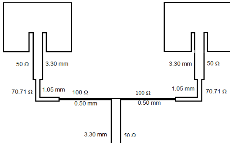
Fig. 9. Schematic Diagram of Cooperate-fed 1 x 2 Antenna Array
