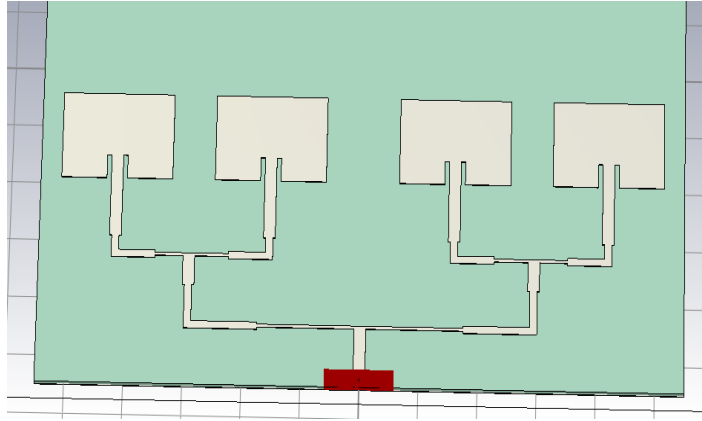
Fig. 12. Model 1 x 4 Cooperate-fed MSA Array
