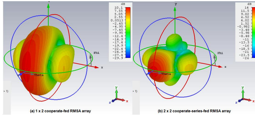
Fig.28. 3-D gain of proposed 1 x 2 cooperate-fed and 2 x 2 cooperate-series-fed RMSA array at 2.4 GHz
