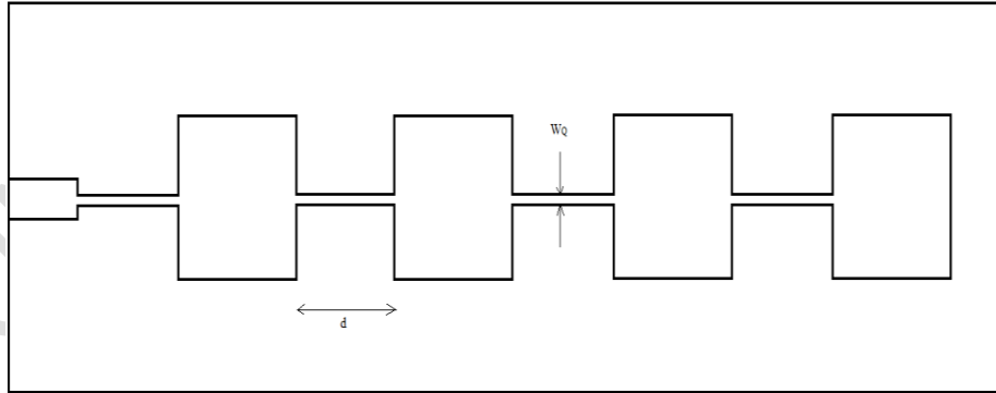
Fig. 3. Schematic diagram of series-fed 1 x 4 patch antenna array
