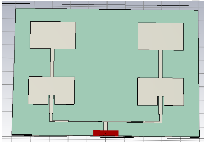
Fig. 13. Model of 2 x 2 Cooperative-series-fed 2 x 2 MSA Array
