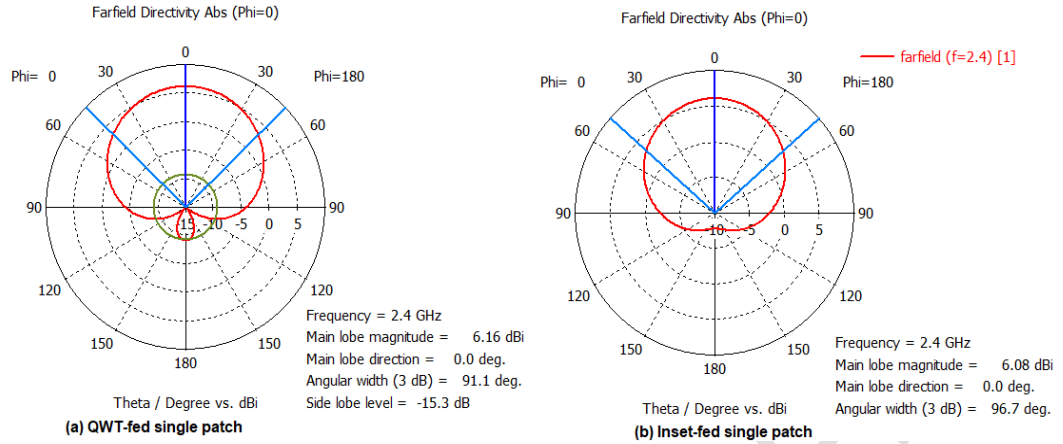
Fig.23. Directivity of single band antenna at 2.4 GHz in E-plane ( \phi = 0^\circ )
