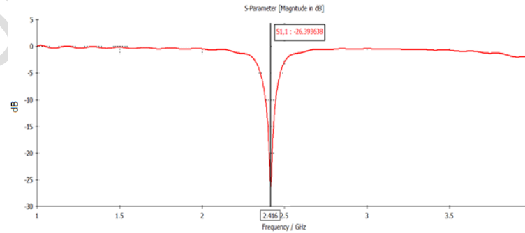
Fig. 16. Return Loss plot of inset-fed single band antenna
