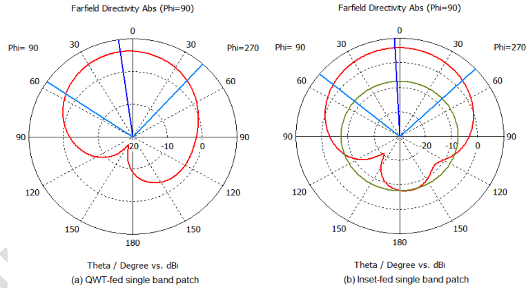
Fig.20. Directivity of single band antennas at 2.4 GHz in H-plane ( \phi = 90^\circ )
