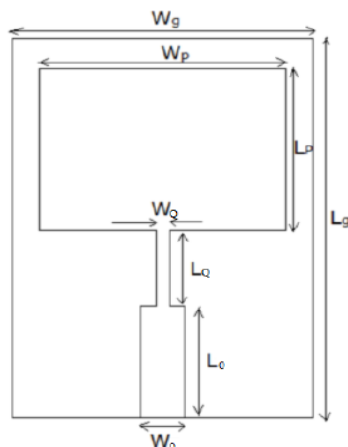
Fig. 1. Schematic diagram of MSA using quarter-wave feed at 2.4 GHz
