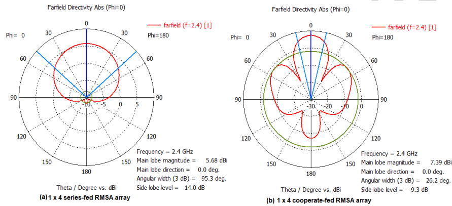
Fig.24. Directivity of array antennas at 2.4 GHz in E-plane ( \phi = 0^\circ )
