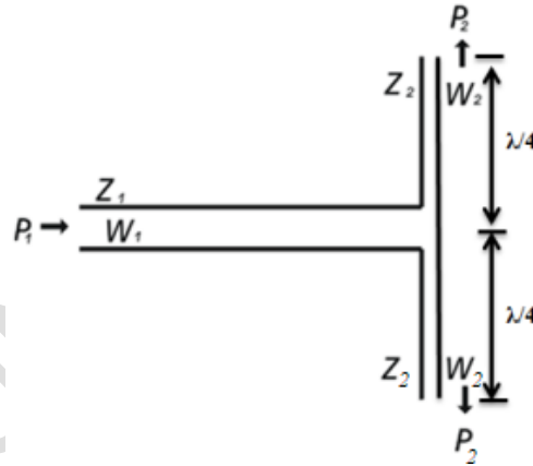
Fig. 7. Microstrip T-junction
