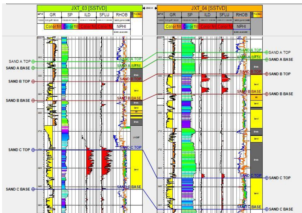
Figure 5: Reservoirs correlated across JXT 03 and 04.
