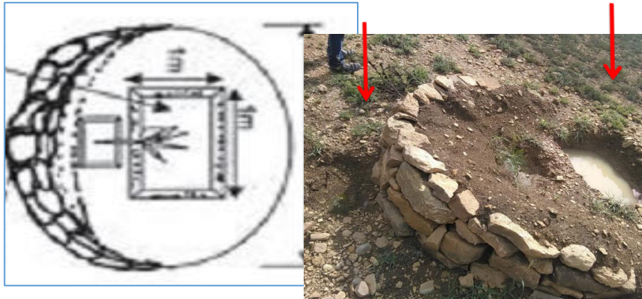
Figure3.Design and constructed eyebrow basin structure
