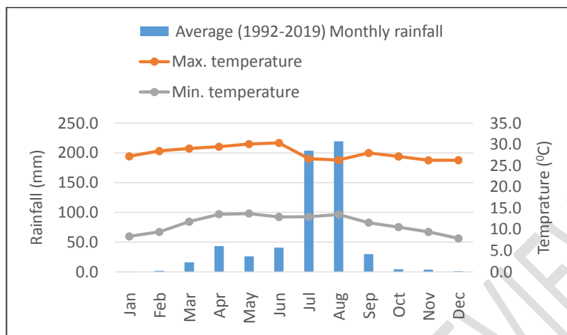
Figure 2. Monthly average rainfall (mm) and temperature (°C) of 27 years
