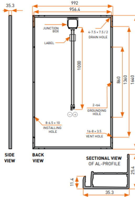
Fig. 2. Dimension of solar module (all the values in mm)
