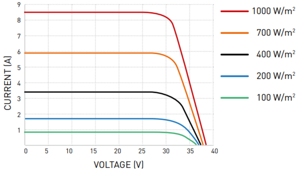
Fig.3 Typical I-V curve of solar module under laboratory condition with different radiation.
