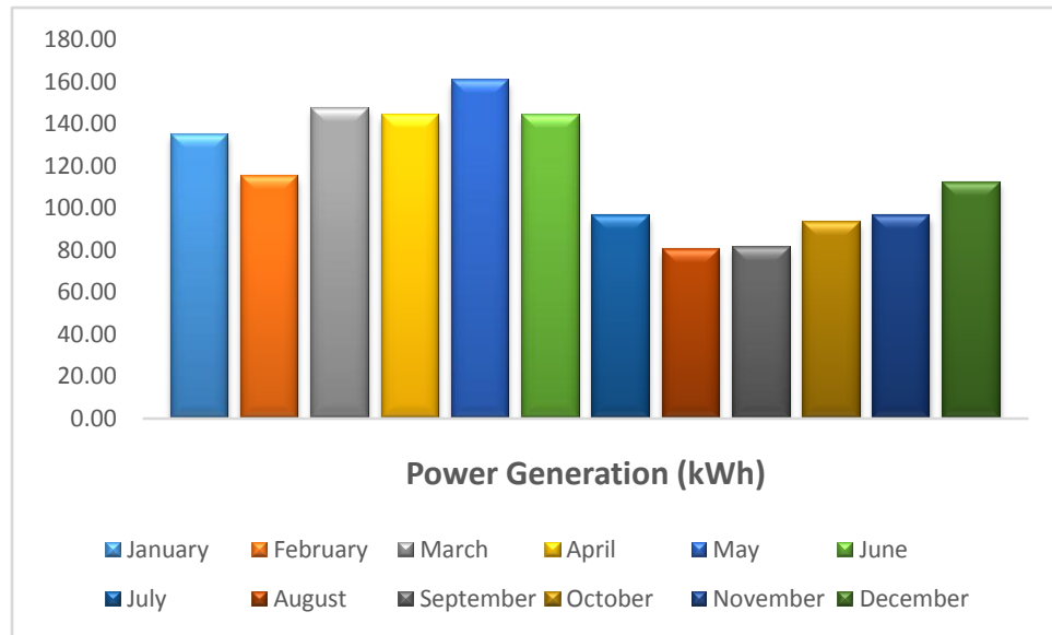
Fig. 4: Monthly energy generation for different months from solar roof top power plant
