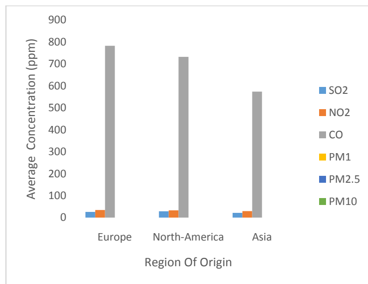
Figure 3: Truck emission according to Region of Origin
