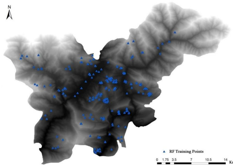
Fig. 5. RF training points
