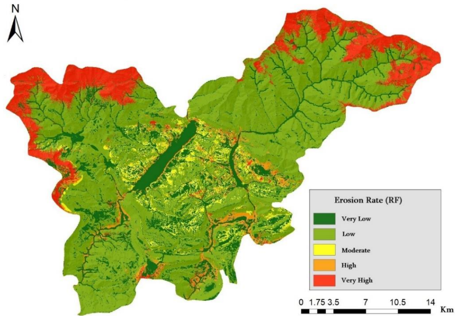
Fig. 8. Spatial distribution of soil erosion in the study area (as a result of RF modeling)
