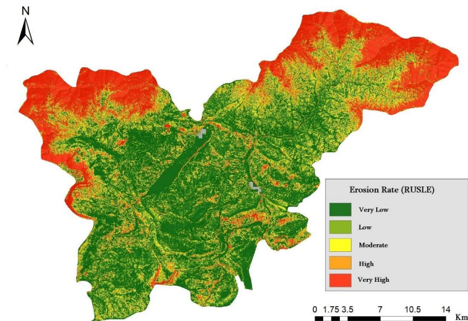
Fig. 6. Spatial distribution of soil erosion in the study area (as a result of RUSLE modeling)
