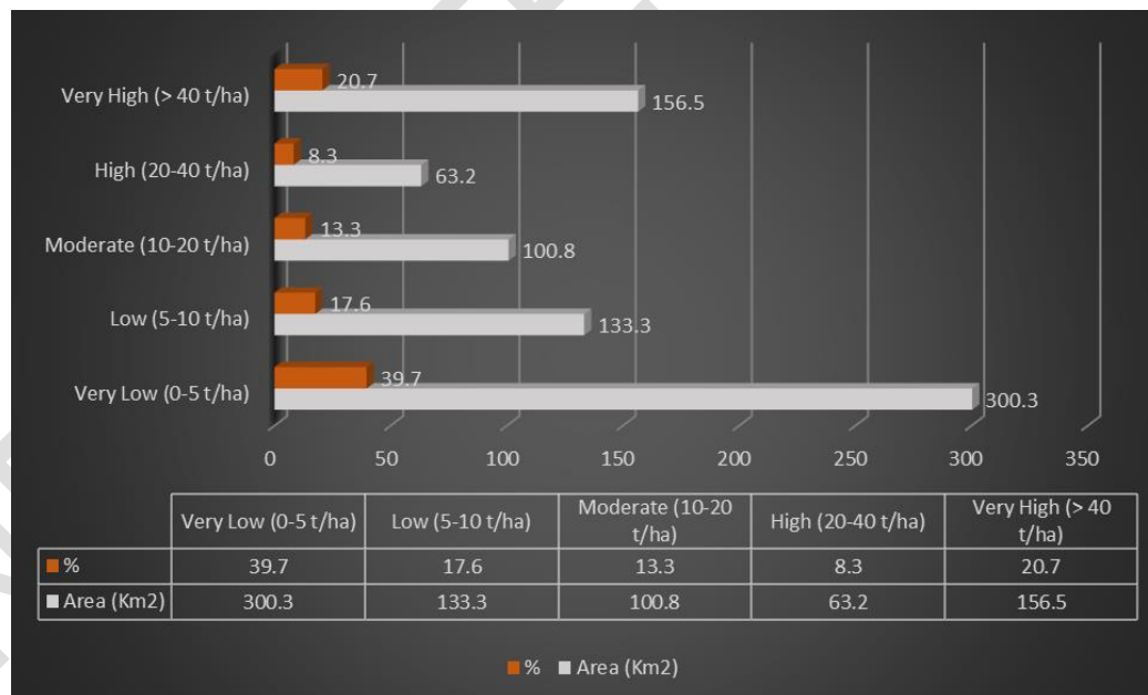
Fig. 7. Distribution of soil loss by area (RUSLE)
