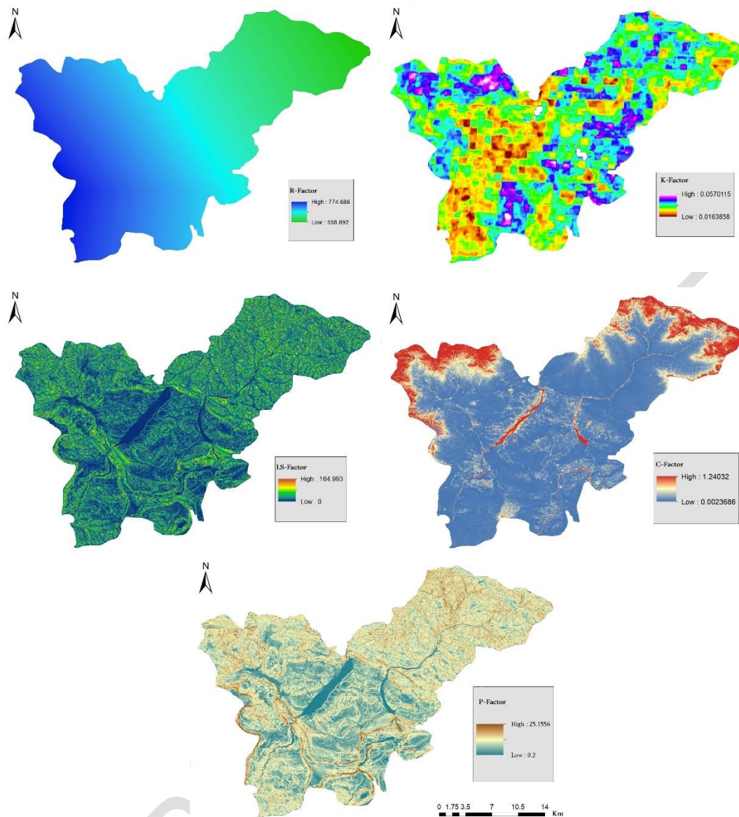
Fig. 3. RUSLE factors. From left to right: R factor; K factor; LS factor; C factor; P factor
