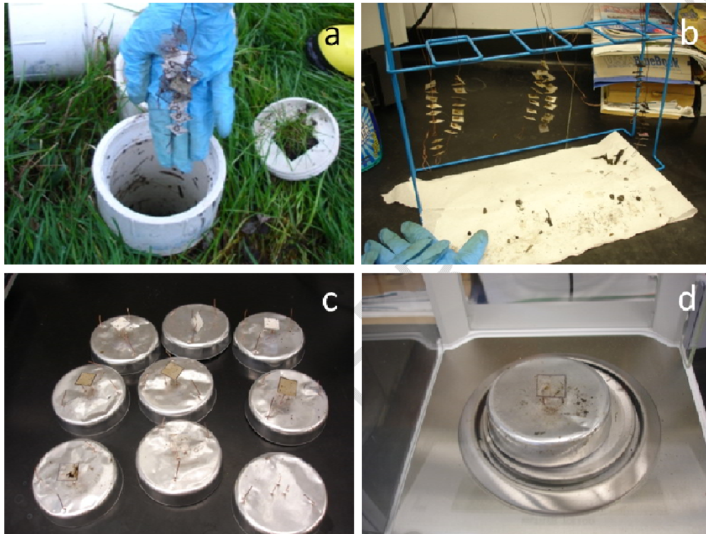
Fig. 8: Test Specimen Examination, a) sample recovery, by drying of samples, c) storage of samples, d) weighting of samples.
