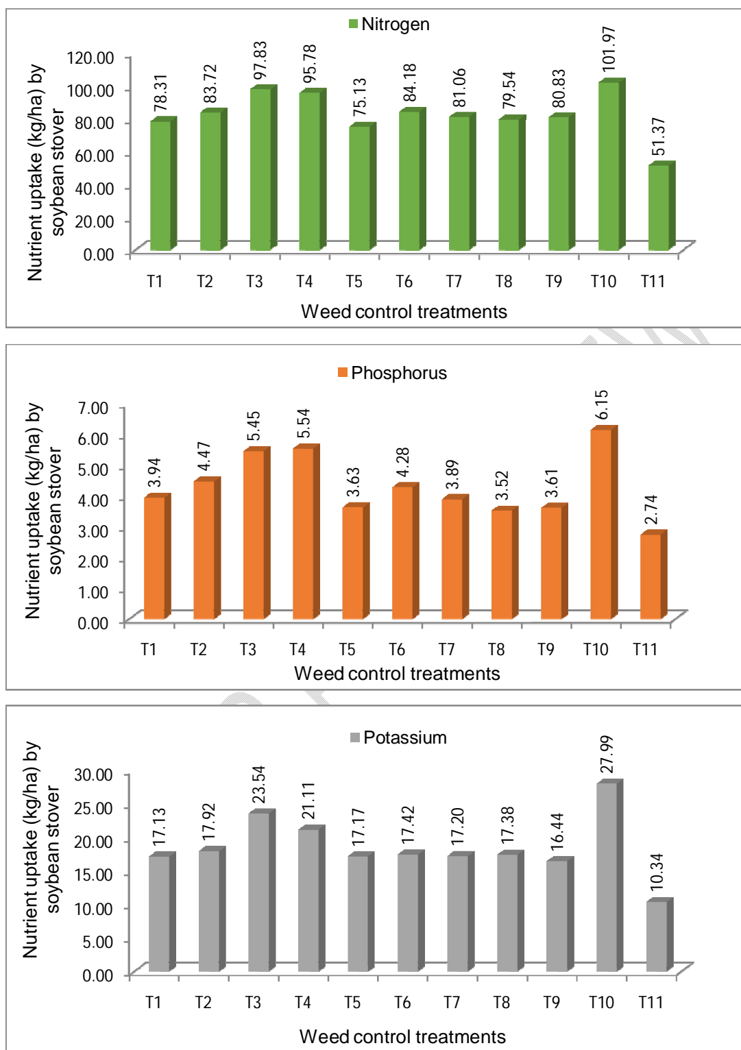
Fig.5 Effect of treatment on nutrient uptake (kg/ha) by soybean stover
