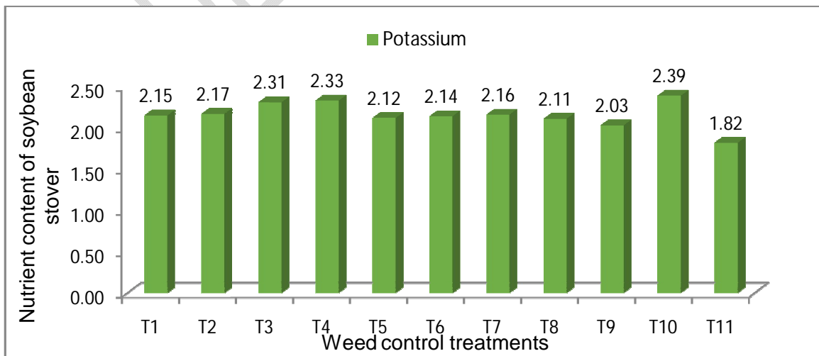
Fig.3 Effect of treatments on nutrient content of soybean stover
