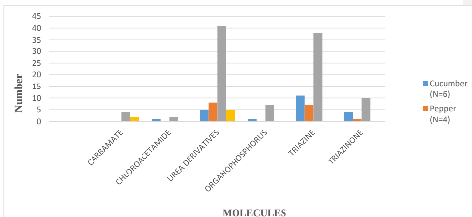
Figure 6 : Families of pesticides found in plants
