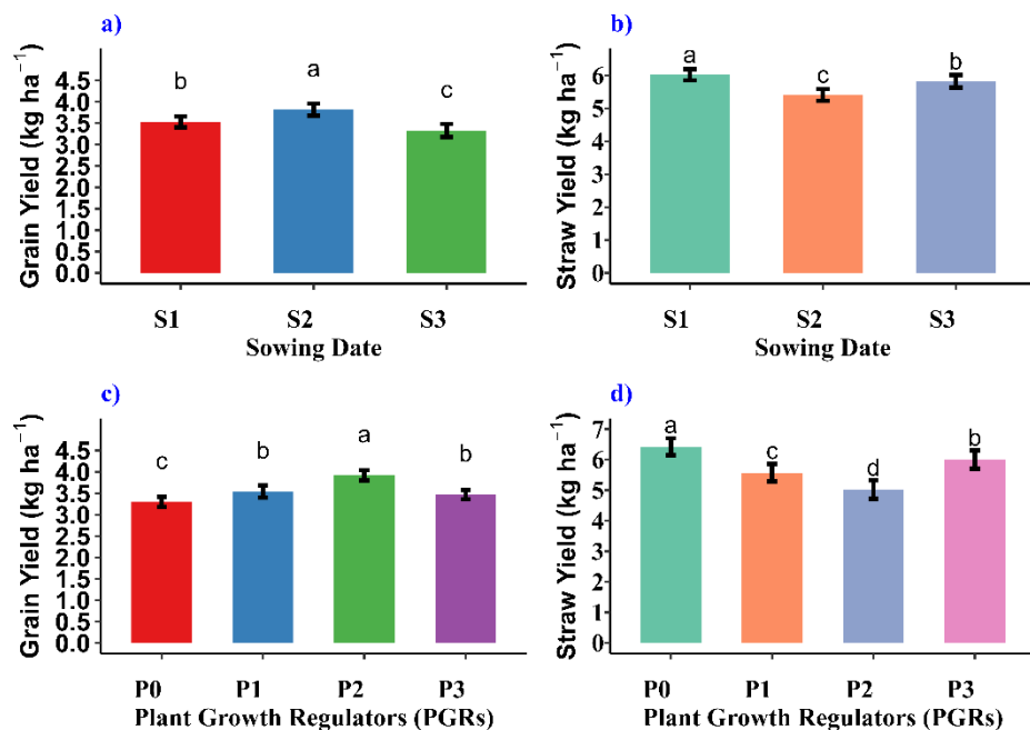
Figure 4. Yield parameters of wheat as influenced by sowing date and PGRs. a) Grain yield affected by sowing date; b) Straw yield affected by sowing date; c) Grain yield affected by PGRs; d) Straw yield affected by PGRs (Data are presented as mean \pm SEm , n = 3; \alpha=0.05 ) (S 1 = 20 th November; S 2 = 5 th December; S 3 = 20 th December) (P 0 = Water only; P 1 = IAA; P 2 = GA 3 ; P 3 = NA)
