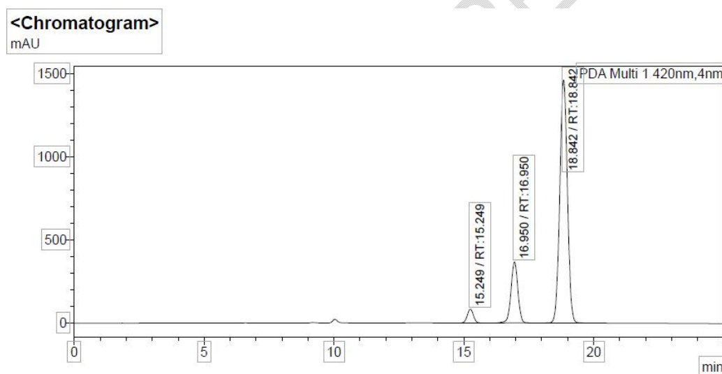
Figure 4: HPLC Chromatogram of regular marketed Curcumin 95% .
