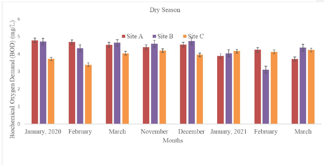
Figure 12: Dry season mean Biochemical Oxygen Demand (BOD) mg/L variation of River Benue at Lau, Mayo-ranewo, and Ibi (2020-2021). Site A Lau, Site B Mayo-ranewo, and Site C Ibi
