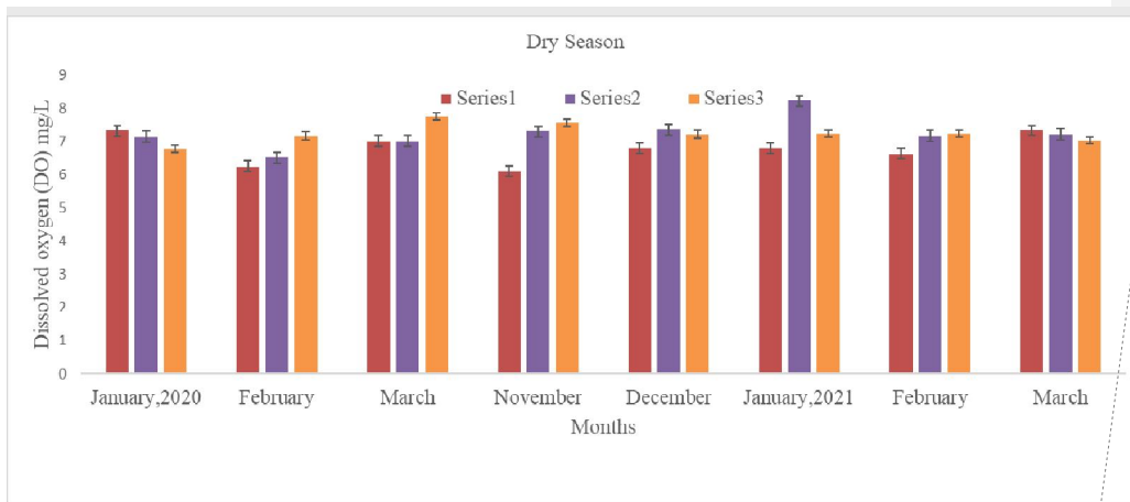
Figure10: Dry season mean Dissolved oxygen (DO) mg/L variation of River Benue at Lau, Mayo-ranewo, and Ibi (2020-2021). Site A Lau, Site B Mayo-ranewo, and Site C Ibi
