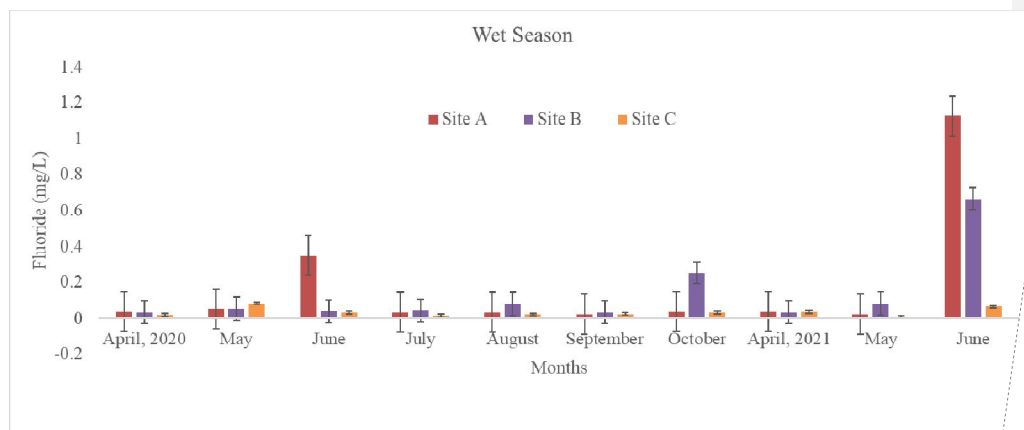
Figure 19: Wet season mean Fluoride (mg/L) variation of River Benue at Lau, Mayo-ranewo, and Ibi (2020-2021). Site A Lau, Site B Mayo-ranewo, and Site C Ibi
