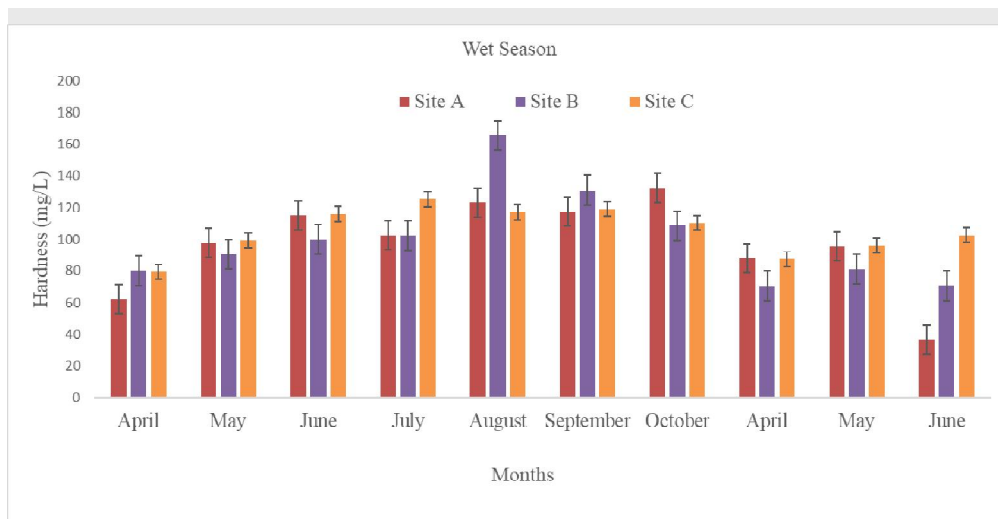
Figure 17: Wet season mean Hardness (mg/L) variation of River Benue at Lau, Mayo-ranewo, and Ibi (2020-2021). Site A Lau, Site B Mayo-ranewo, and Site C Ibi
