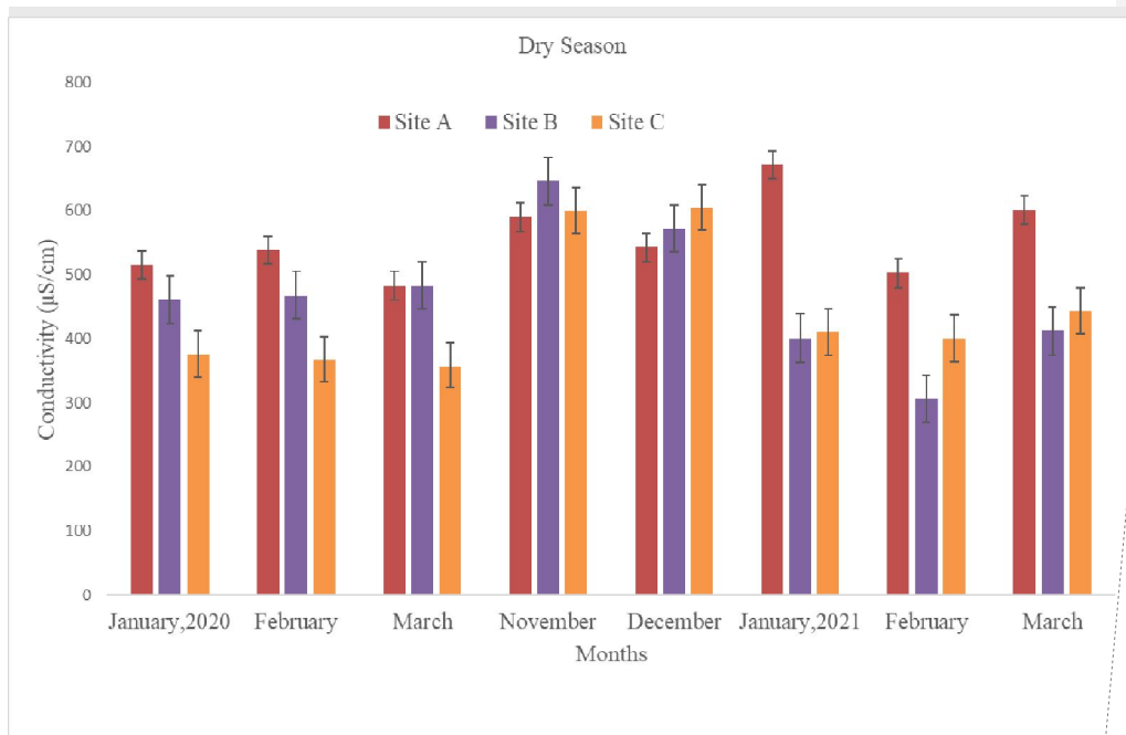
Figure 8: Dry season mean Conductivity ( \mu\text{S}/\text{cm} ) variation of River Benue at Lau, Mayo-ranewo, and Ibi (2020-2021). Site A Lau, Site B Mayo-ranewo, and Site C Ibi
