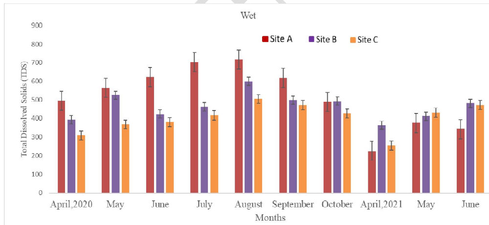
Figure 7: Wet season mean Total Dissolved Solids (TDS) mg/L variation of River Benue at Lau, Mayo-ranewo, and Ibi (2020-2021).Site A Lau, Site B Mayo-ranewo, and Site C Ibi
