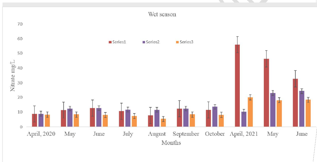
Figure 21: Wet season mean Nitrate (mg/L) variation of River Benue at Lau, Mayo-ranewo, and Ibi (2020-2021). Site A Lau, Site B Mayo-ranewo, and Site C Ibi
