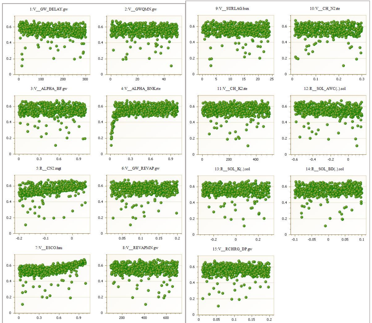
Fig. 9 Dotty plots of SWAT parameters range against the objective function of NSE
