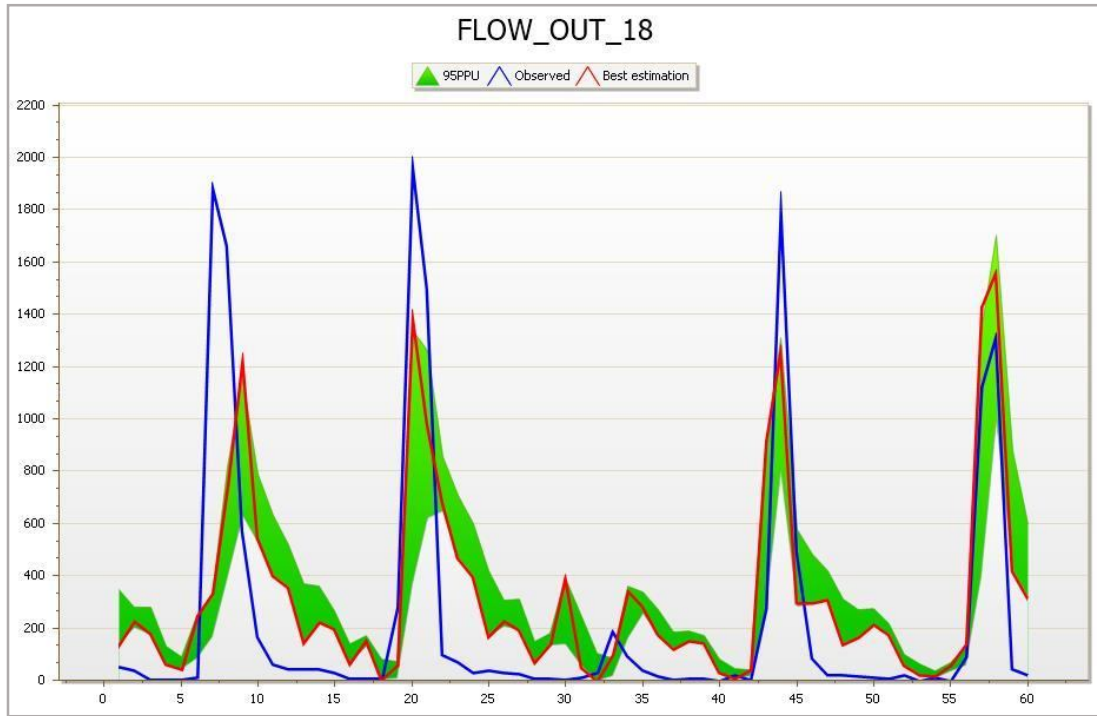
(b) Fig. 11 Observed, simulated stream flow and 95 % probability uncertainty plot during (a) calibration (2003–2011) and (b) validation (2013–2017) at Huvenhedgi gauging station.
