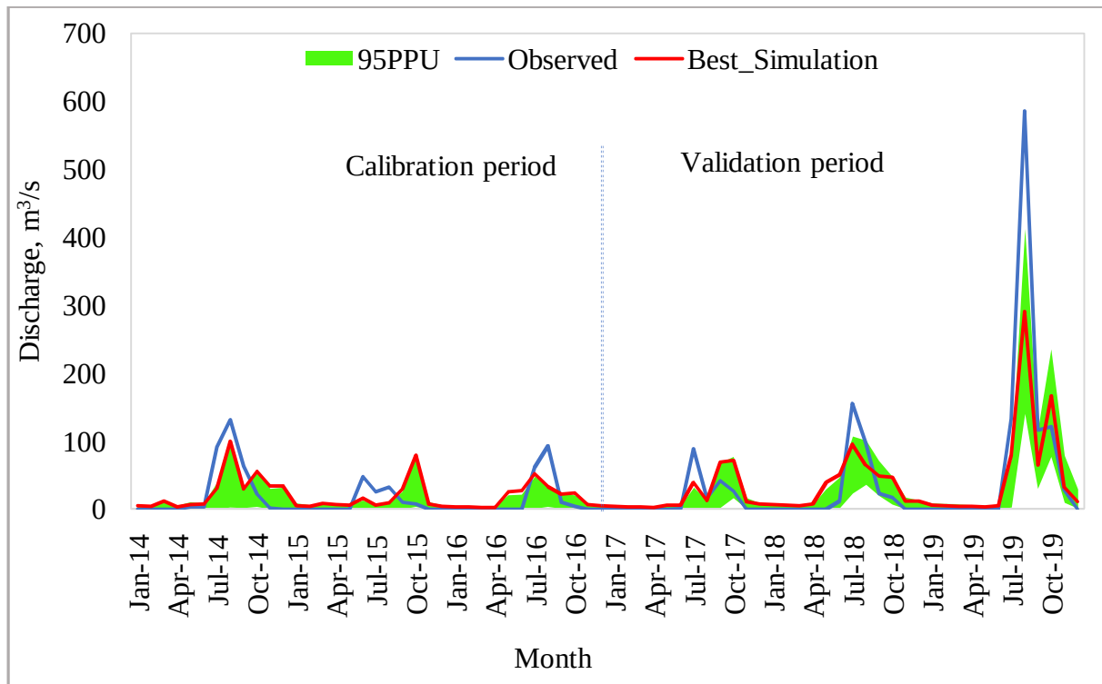
Fig. 13 Observed, simulated stream flow and 95PPU during calibration and validation period at Malaprabha (Renukasagar) dam gauging station
