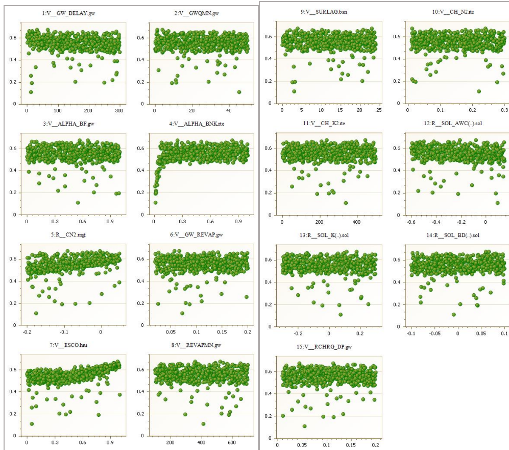
Fig. 9 Dotty plots of SWAT parameters range against the objective function of NSE
