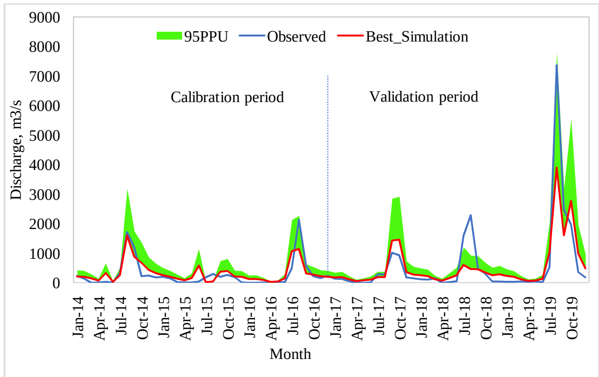
Fig. 15 Observed, simulated stream flow and 95PPU during calibration and validation period at Narayanpur dam gauging station
