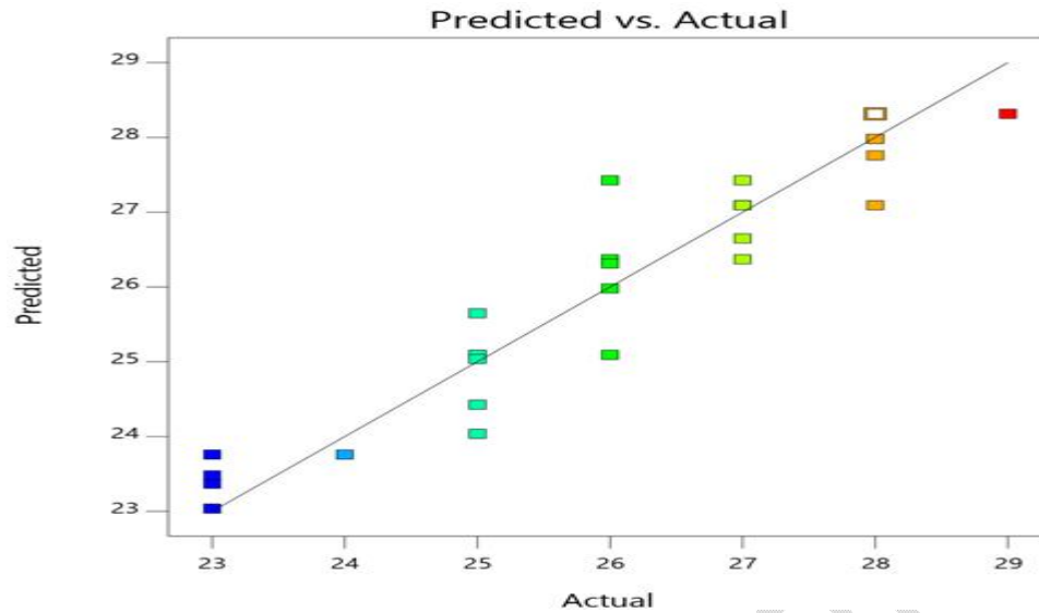
Fig 1 Diagnostics plots of the fitted quadratic model for soil temperature
