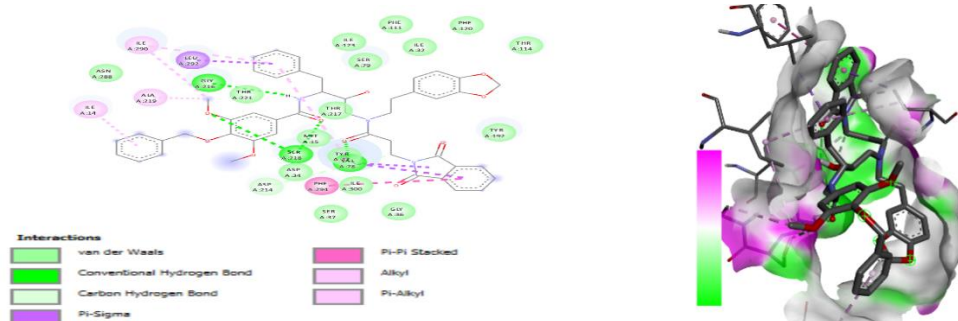
Figure 2a: Molecular interaction of amino acid residue of plasmepsin with EH58, 2D left 3D right.
