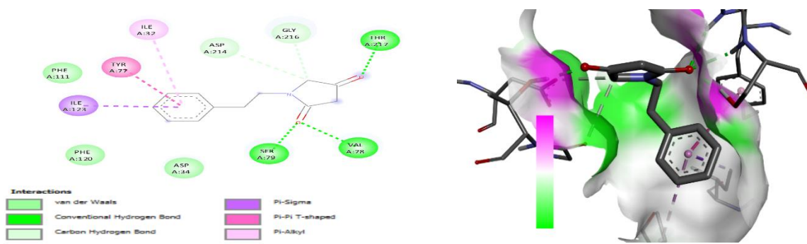
Figure 2c: Molecular interaction of amino acid residue of plasmepsin with 3-benzyl-6-methylpiperazine-2,5-dione, 2D left 3D right.
