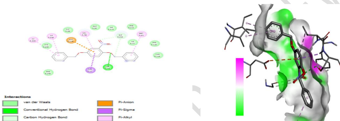
Figure 2b: Molecular interaction of amino acid residue of plasmepsin with 2,5-dibenzoyloxynitrobenzene, 2D left 3D right.
