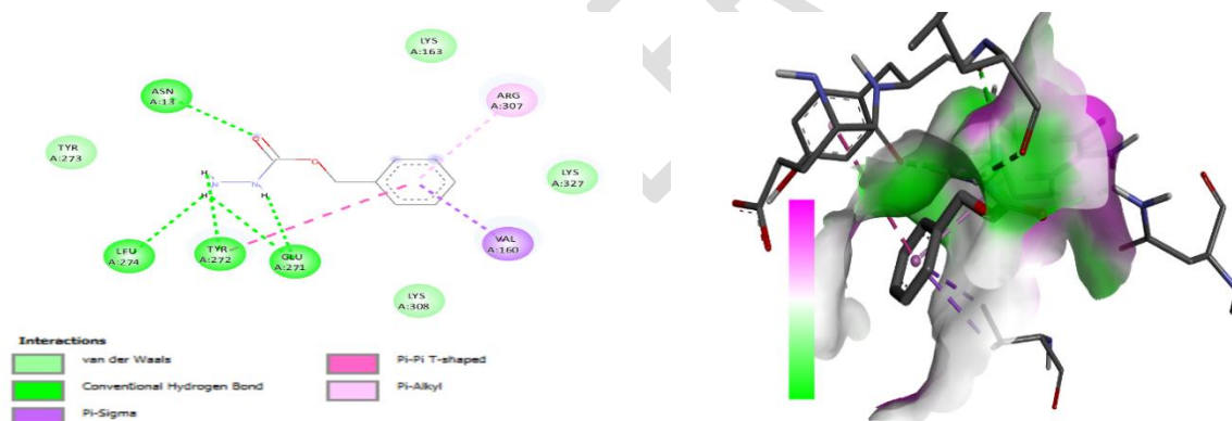
Figure 2f: Molecular interaction of amino acid residue of plasmepsin with Benzylhydrazine carboxylat, 2D left 3D right.
