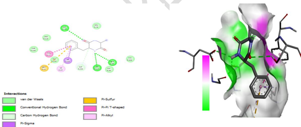
Figure 2c: Molecular interaction of amino acid residue of plasmepsin with 3-benzyl-6-methylpiperazine-2,5-dione, 2D left 3D right.
