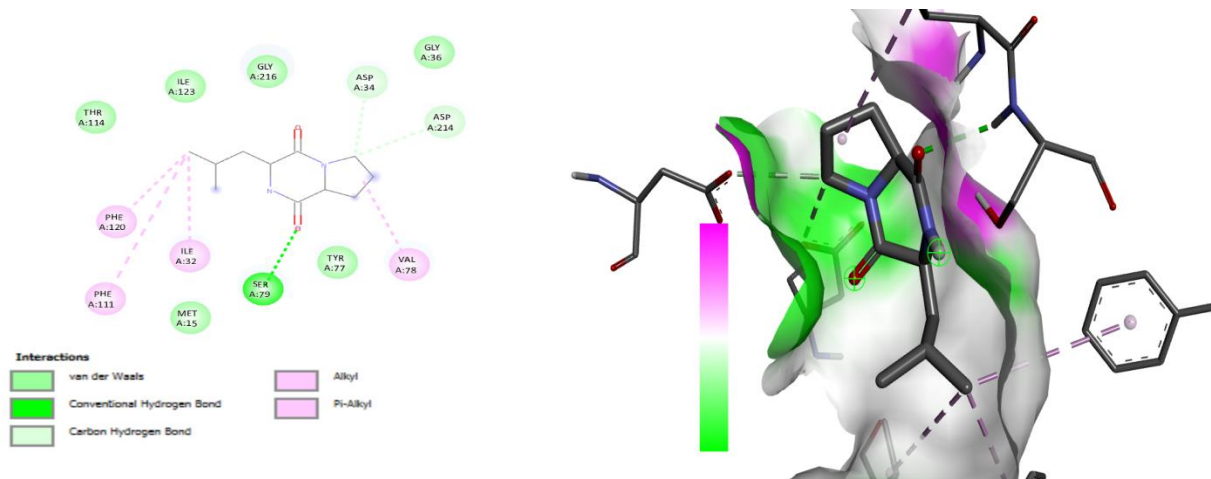
Figure 2e: Molecular interaction of amino acid residue of plasmepsin with pyrrolo[1,2-a]pyrazine-1,4-dione, hexahydro-3-(2-methylpropyl)-, 2D left 3D right.
