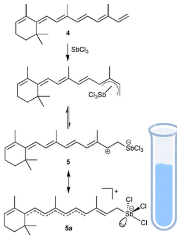
Fig . 31 . Reaction and result - Carr-Price reaction
