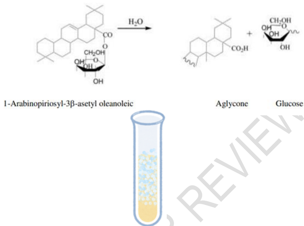
Fig . 30 . Reaction and result - Shake test
