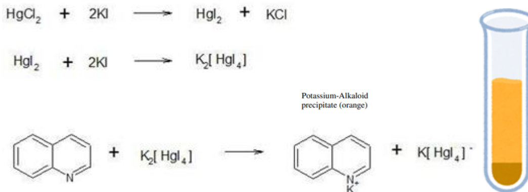
Fig .18 . Reaction and result - Mayer's test
