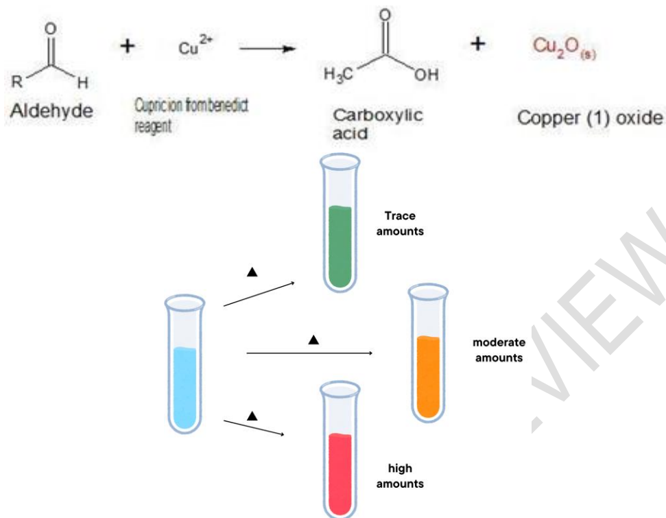
Figure . 3 . Reaction and result - Benedict's test
