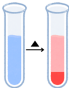
Figure . 5 . Reaction and result - Barfoed's test
