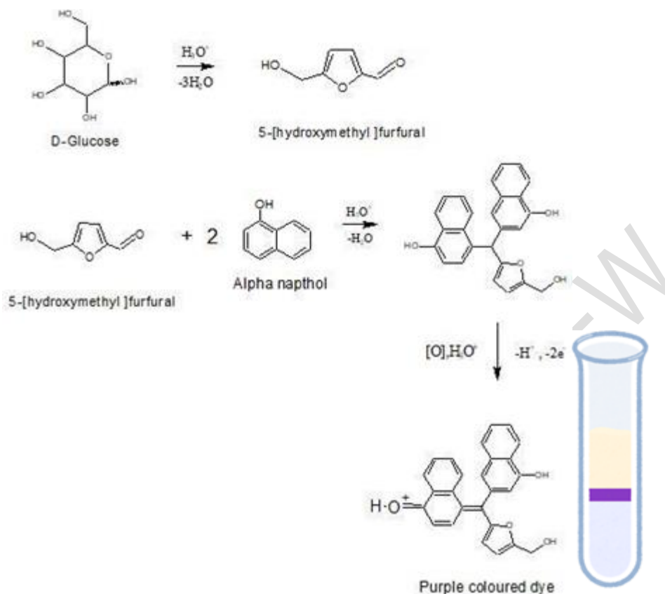
Fig . 2 .Reaction and result - Molisch test
