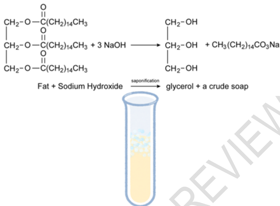
Fig . 34, Reaction and result - Saponification test
