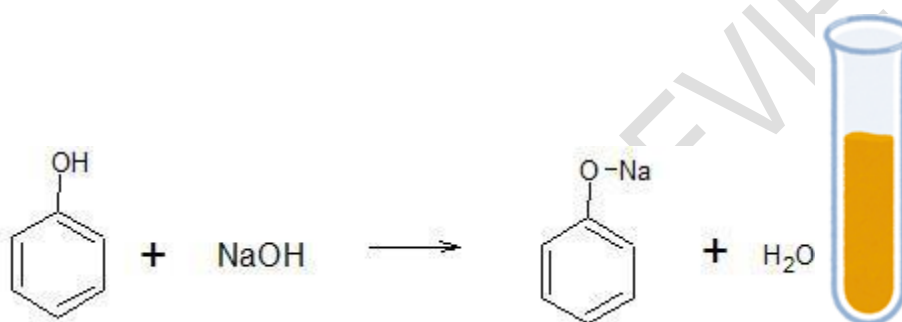
Fig . 23. Reaction and result - Alkaline reagent test
