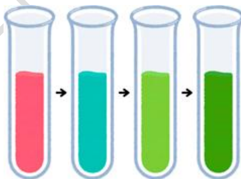
Fig . 27 . Reaction and result - Liebermann- Burchard test
