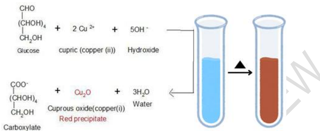
Figure . 4 . Reaction and result - Fehling's test
