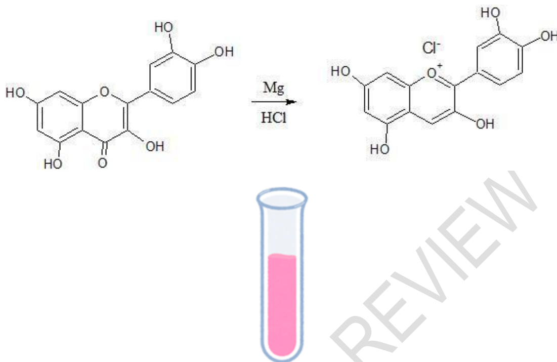
Fig . 24. Reaction and result - Shinoda's test
