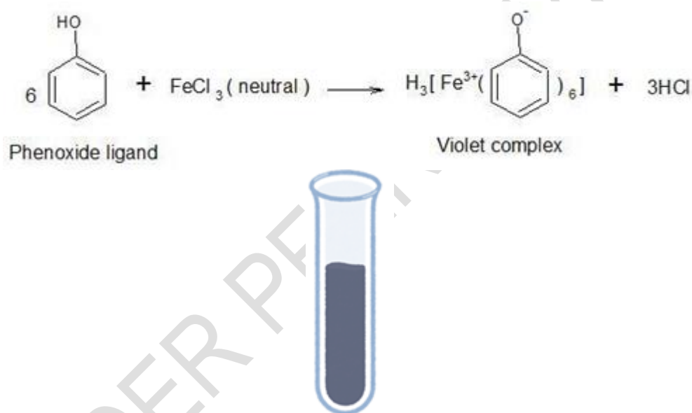
Fig . 22 .Reaction and result - Ferric chloride test
