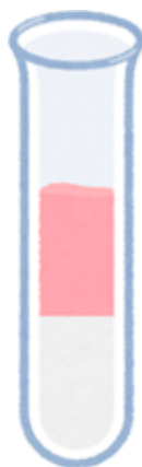
Fig . 15 . Reaction and result - Borntrager's test
