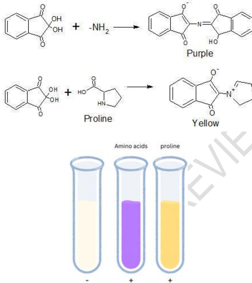
Fig . 10 . Reaction and result - Ninhydrin test
