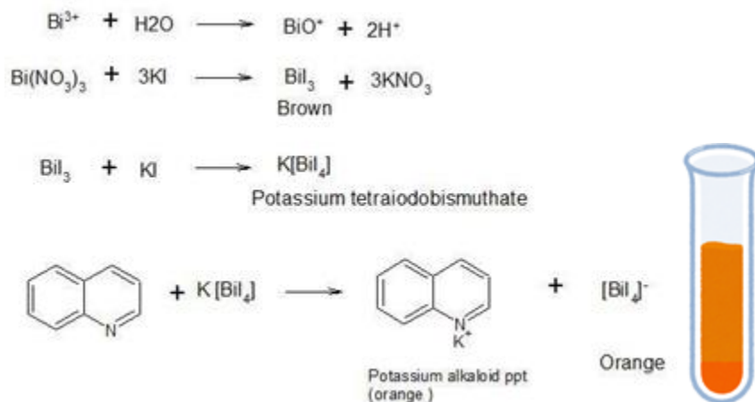
Fig . 20 . Reaction and result - Dragendorff's test
