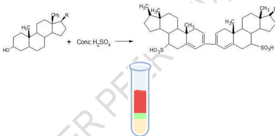
Fig .28 .Reaction and result - Salkowski's test
