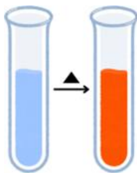
Figure . 6 . Reaction and result - Trommer's test
