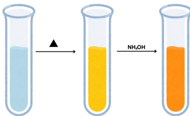
Fig . 13 . Reaction and result - Xanthoproteic test
