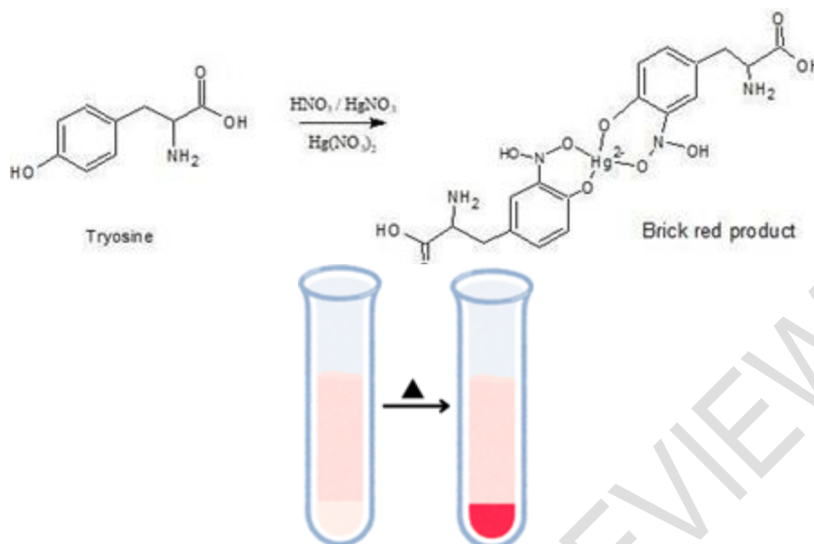
Fig . 9 . Reaction and result - Millon's test
