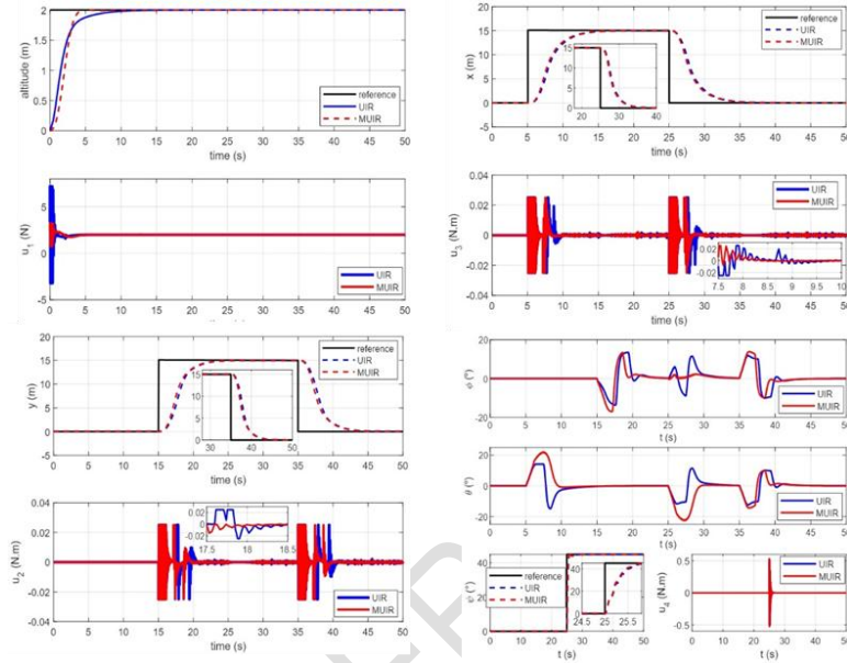
Fig.3.Altitude, X-position, Y-position and Attitude quadrotor response
