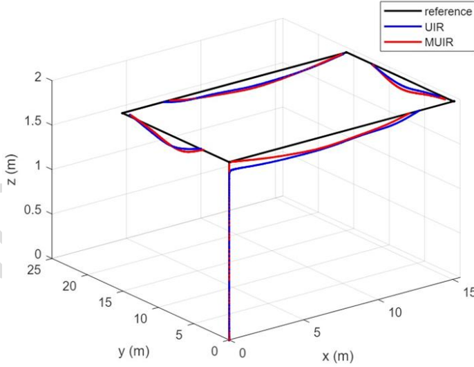
Fig.2.3D quadrotor square trajectory
