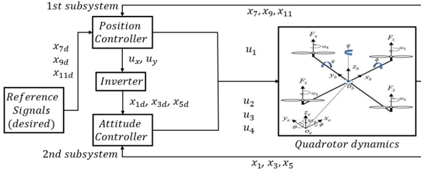
Fig.1. Quadrotor control structure
