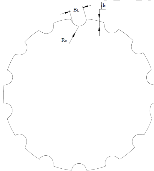
Fig. 1: Vertical rotor cell design parameters
