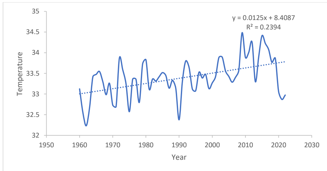
Fig.2. Trend of annual Temperature of Telangana from 1960-2022
