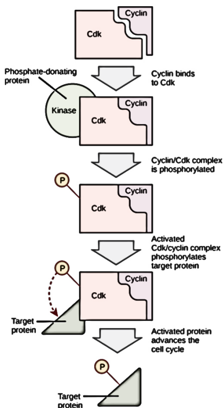
Fig. 3. Cyclin-dependent kinases(3)
