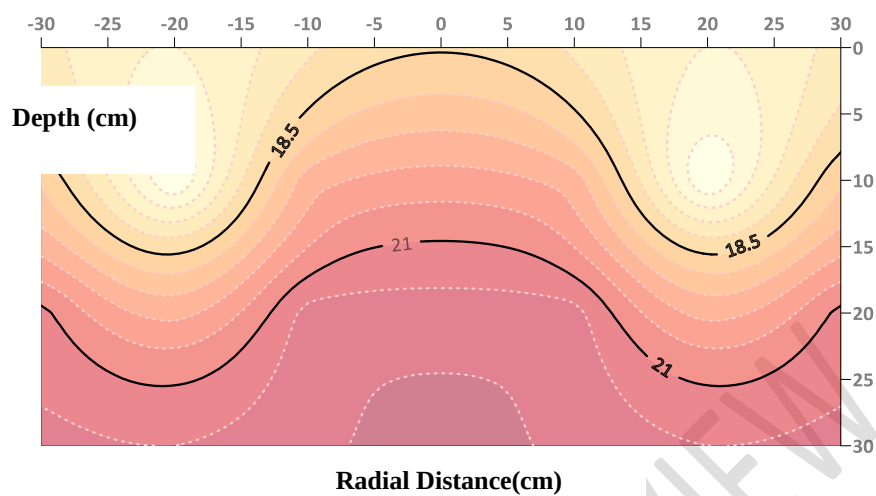
Fig.2 Soil moisture distribution at 24 hr after irrigation
