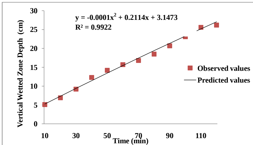
Fig 6 Time V/s Vertical wetted zone depth
