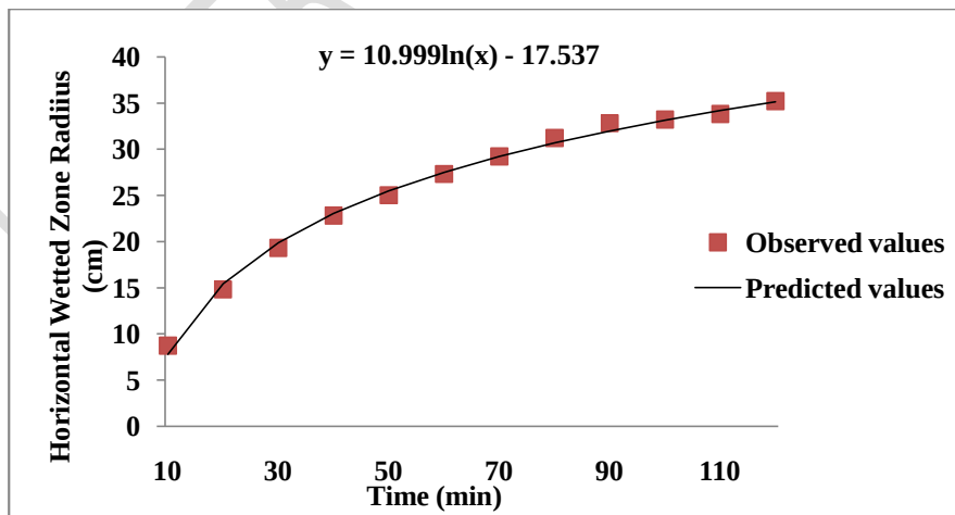
Fig 5 Time V/s Horizontal wetted zone radius
