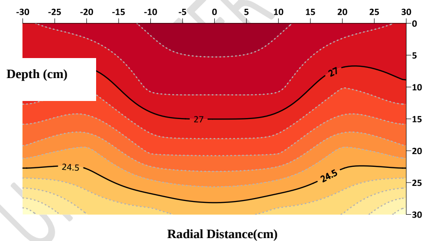
Fig.1 Soil moisture distribution at 2 hr after irrigation
