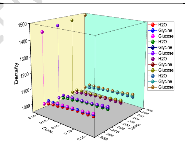
Fig.2 Density
