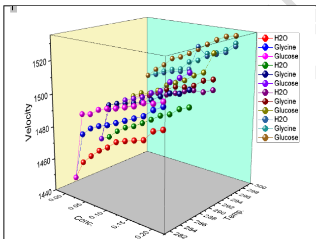
Fig. 1 Ultrasonic Velocity
