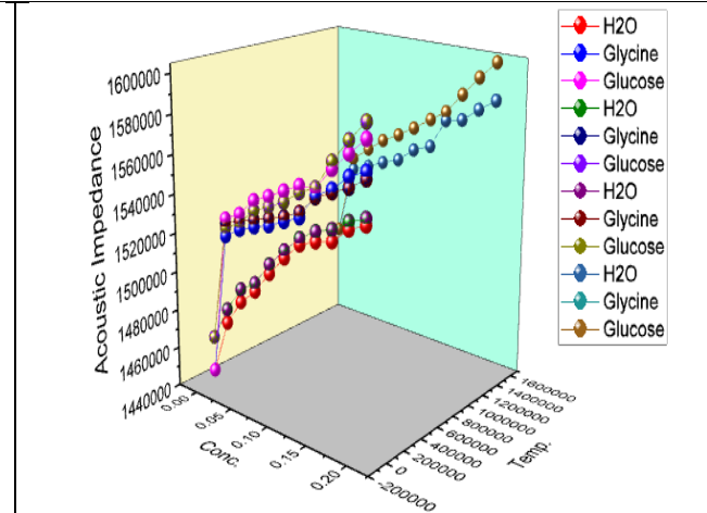
Fig.4 Acoustic impedance
