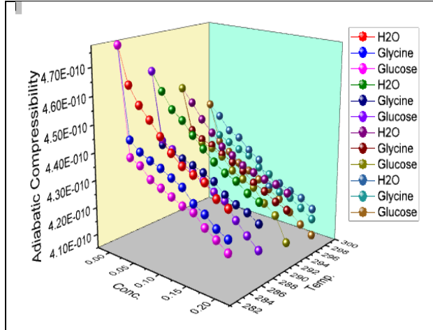
Fig.3 Adiabatic Compressibility
