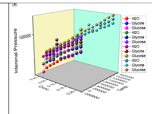
Fig.10 Internal pressure
