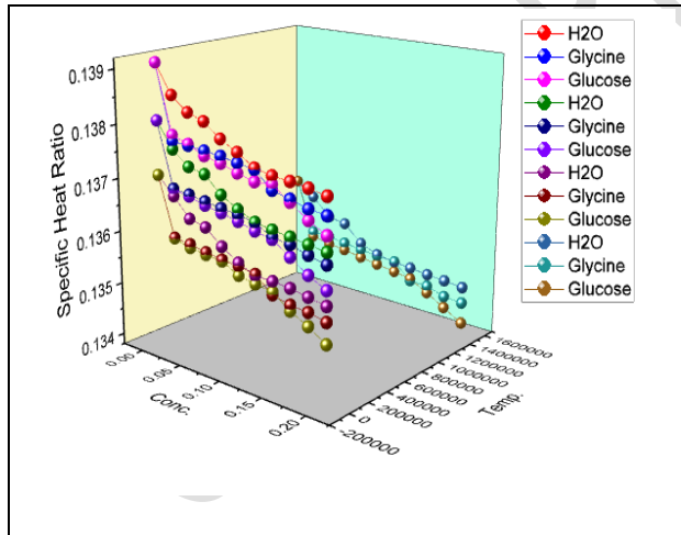
Fig.5 Specific Heat Ratio
