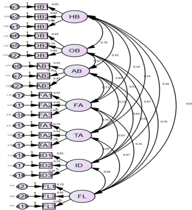
Figure 2. Structural equation model
