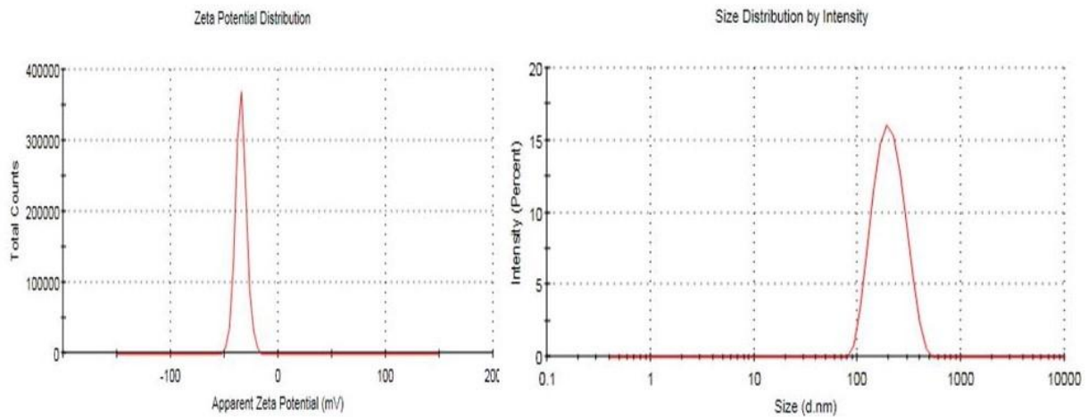
Fig 7 a) Zeta Potential and surface charge b) Average size distribution of PVP conjugated AuNPs
