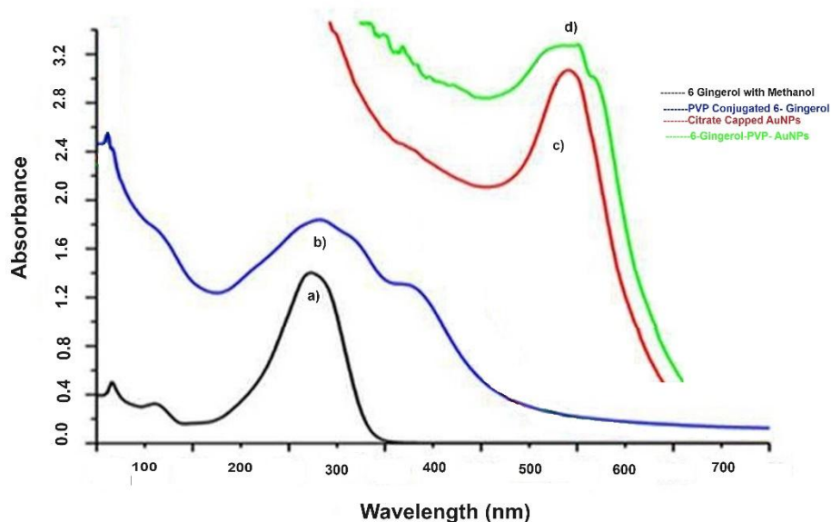
Fig.1 : UV-Vis Spectrum of Au-PVP-6-Gingerol Conjugates in various stages
