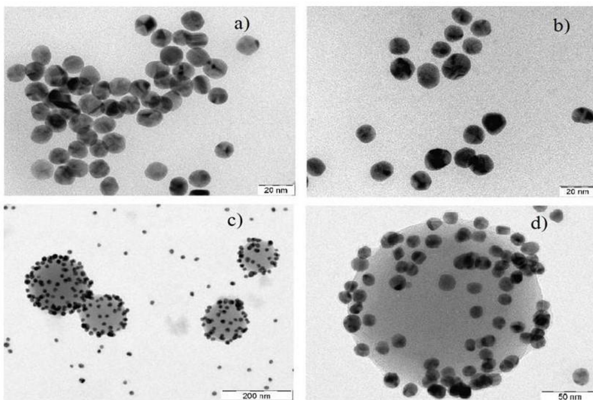
Fig. 5- HR-TEM images of a) AuNPs, b) PVP capped AuNPs, c) 6-Gingerol-PVP-AuNPs d) Magnify images of conjugated NPs.
