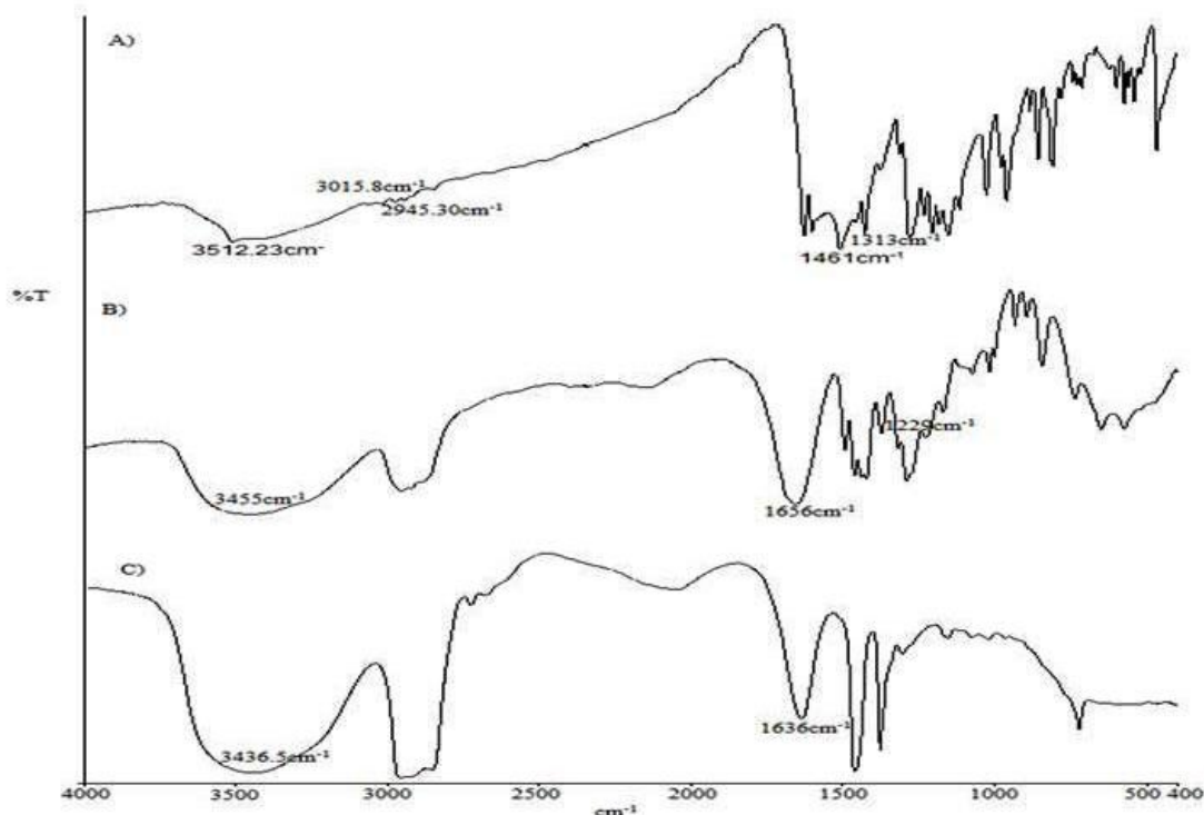
Figure 2: FTIR spectrum of a) 6-Gingerol, b) PVP capped AuNPs, c) Conjugated AuNPs-PVP-6-Gingerol
