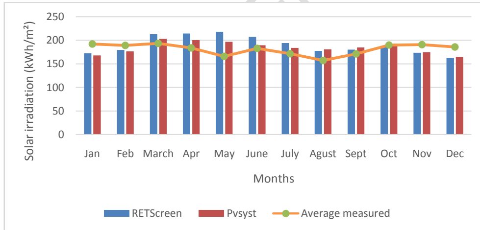
Fig. 1 : Simulated monthly irradiance and average irradiance measured from 2019 to 2021. The monthly and annual electricity production values obtained from the simulations using the PVsyst and RETScreen programs were compared with the actual power plant values on a monthly and annual basis. The comparison of electricity production data from PVsyst, RETScreen and the power plant is presented in Table 3.
