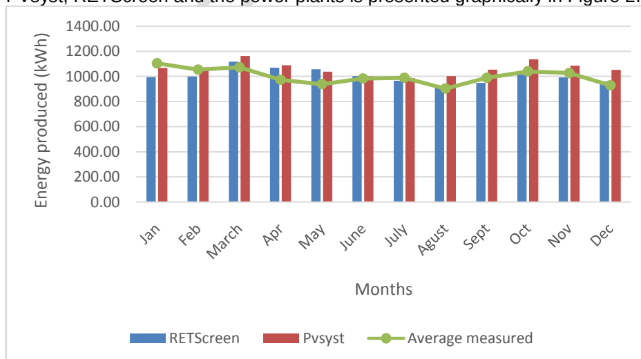
Fig. 2: Simulated monthly energy and average energy measured from 2019 to 2021.
