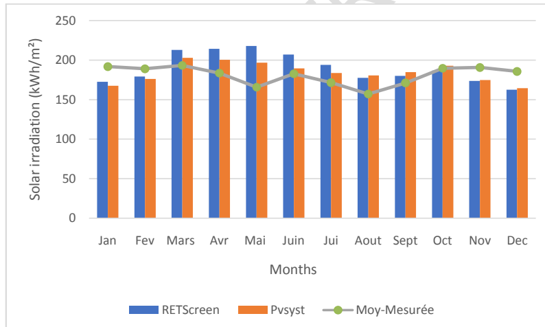
Fig.1 : Simulated monthly irradiance and average irradiance measured from 2019 to 2021.
