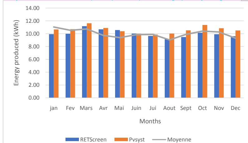
Fig. 2: Simulated monthly energy and average energy measured from 2019 to 2021.
