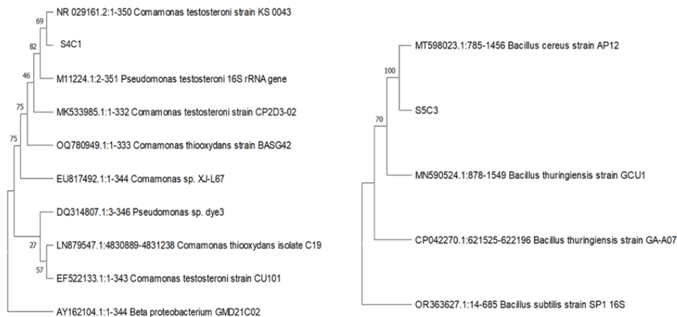
Figure 7: Neighbor joining tree showing the phylogenetic relationship, based on 16S rRNA gene sequences, between the reference bacteria and the identified heavy metal-resistant bacterial isolates S4C1 and S5C3.
