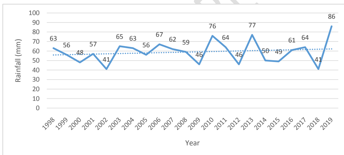
Figure 2: Rainy days (1998-2019)
