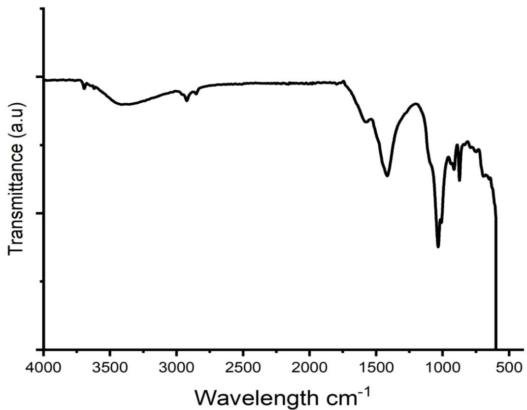
Figure 1. FTIR Spectra of Hydrochar produced from sewage sludge and water hyacinth
