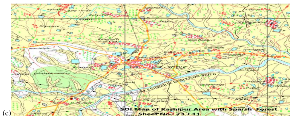
Fig 3:- (a): SOI Purlia District map in 1912 (1:250000scale); (b) SOI of Purlia District map in 1932 ; (c)SOI map of Kashipur Block in 2005 (Gradual diminishing vegetation)
