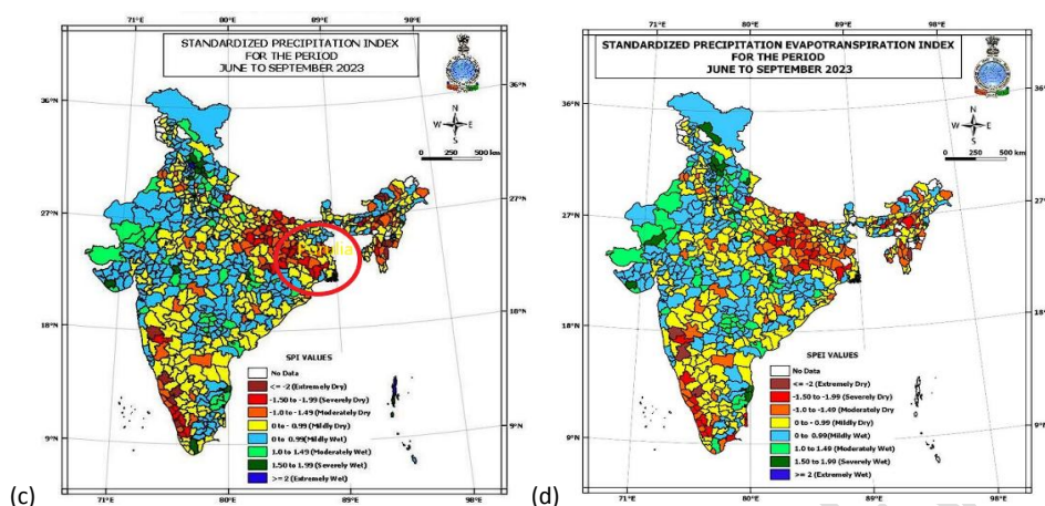
Fig.8:-Drought position during June to Sept 2023; (a)Rainfall departure (%) from Normal (June to Sept. 2023)(b) Mild drought Purulia 2023 as per AAI; ( c) Mild drought in Purulia District (SPI) ; (d) Standardized Precipitation Evapotranspiration Index (SPEI) (Source IMD)
