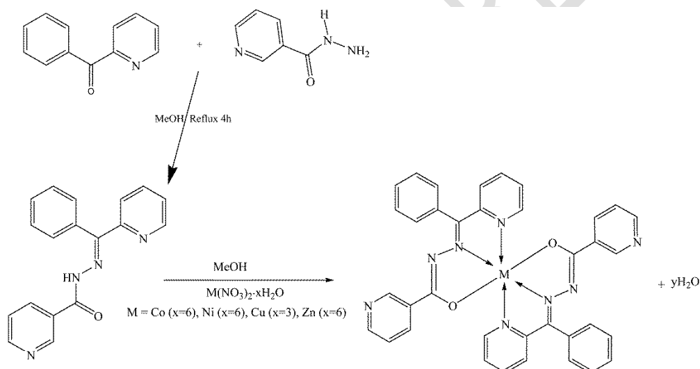
Scheme 1. Synthesis procedure of the ligand HL and its \text{Co}^{2+} , \text{Ni}^{2+} , \text{Cu}^{2+} and \text{Zn}^{2+}
