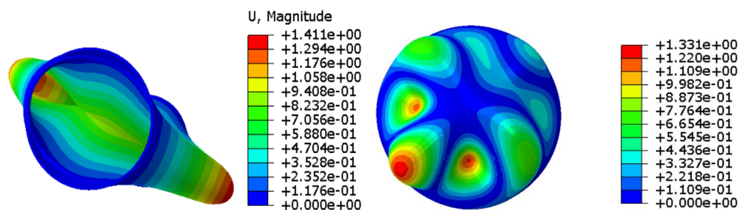
a.Double titanium alloy ballast tank b.Double carbon fiber ballast tank
