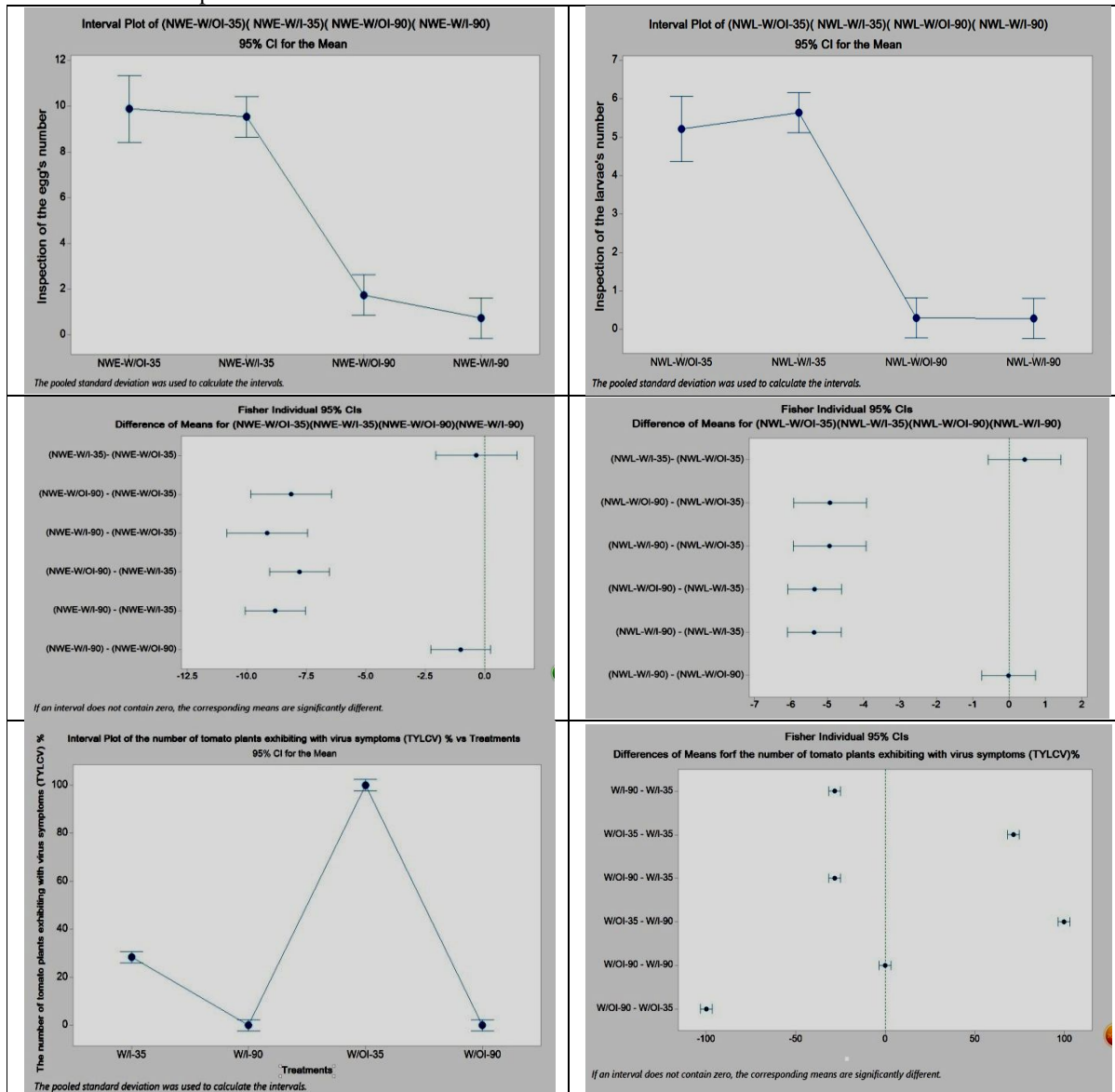
Figure 2. Interval plot and Fisher individual 95% confidence intervals for inspection of the number of whitefly eggs and larvae and the percentage of the number of tomato plants exhibiting virus symptoms (TYLCV) by comparing the different treatments to each other for both procedures for 35-day-old seedlings and 90-day-old transplants.
