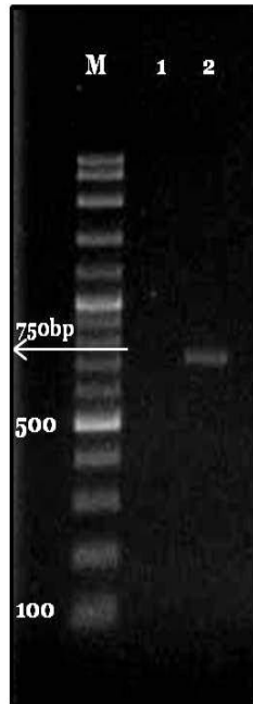
Figure 3. TYLCV amplified product on agarose gel using primers AV1F (5'ATGGCGAAGCGACCAG3') and AV1R (5'TTAATTTGTGACCGAATCAT3'). Molecular detection of tomato yellow leaf curl virus (TYLCV) in tomato seeds; Seeds obtained from both procedures were germinated under a controlled laboratory. The aqueous phase was subjected to agarose gel electrophoresis and stained with ethidium bromide. DNA of sample (2), yielded one band of TYLCV (720 bp), and no PCR products were amplified from samples (1). WHERE, M = marker; sample 1 = a sample of fresh leaves obtained from germinating seeds of the procedure (90-day-old transplants); and sample 2 = a sample of fresh leaves obtained from germinating seeds of the procedure (35-day-old seedlings)
