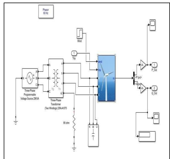
Fig.3.Simulation diagram of Wind turbine
