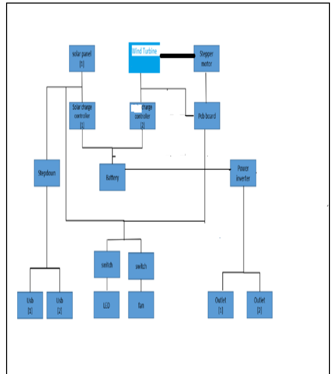
Fig.7. Block diagram for the design of final prototype model
