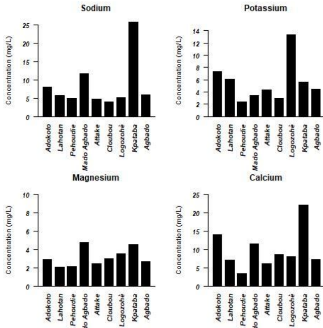
Figure4: Sodium, potassium, magnesium and clacium levels in the waters of the Agbado River
