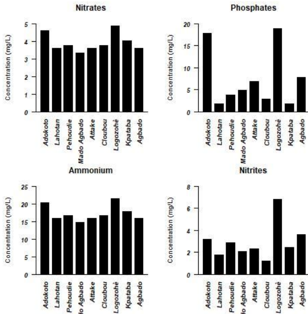
Figure 5: Contents of nitrogen compounds (nitrites, ammonium, nitrates) and phosphorus (phosphates) contained in the waters of the Agbado River
