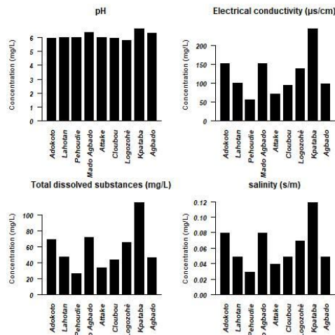
Figure 3: pH, TDS, Conductivity and salinity of the waters of the Agbado River
