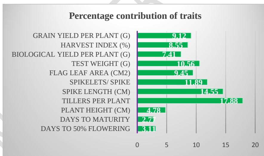
Fig. 2 Trait wise contribution (%) towards total genetic variability
