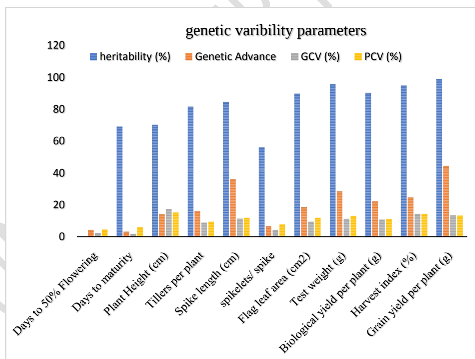
Figure. 1 Genetic variability param
