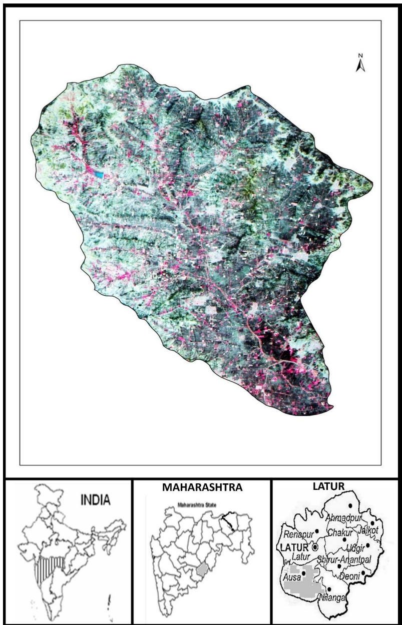
Figure 1: Satallite data of Tungi watershed of Latur district of Maharashtra, India
