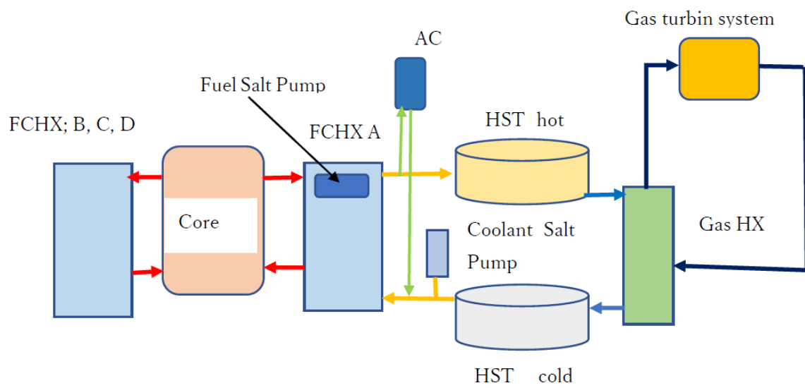
Figure 7. Schematic of a referenced conceptual molten chloride fast reactor [5]; Reproduced by the authors
