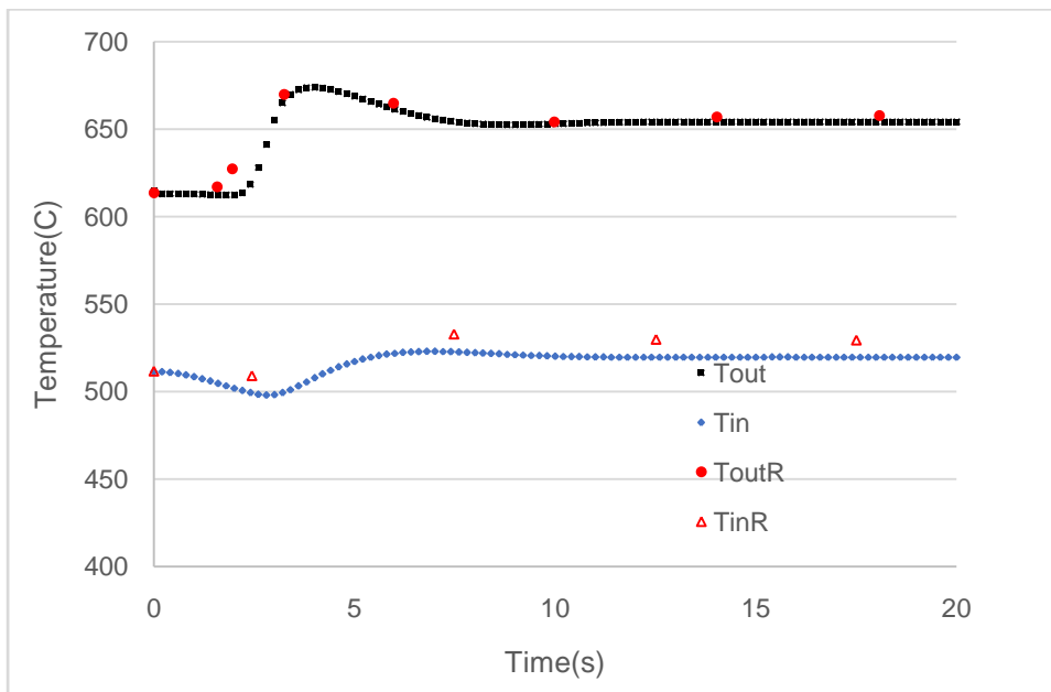
(a) Relative power and fuel flow-rate
