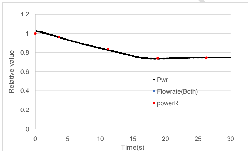
(b) Relative power and fuel flow-rate
